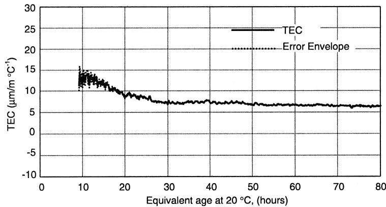
Fig. 12. Thermal expansion coefficient (TEC), Test 4.
