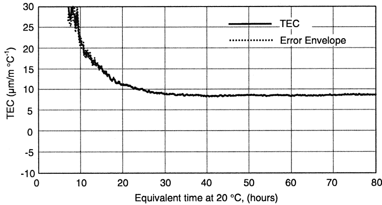
Fig. 11. Thermal expansion coefficient (TEC), Test 3.
