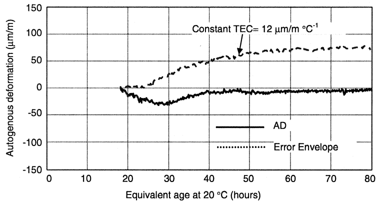
Fig. 21. Autogenous deformation, Test 4: positive values are contractions.
