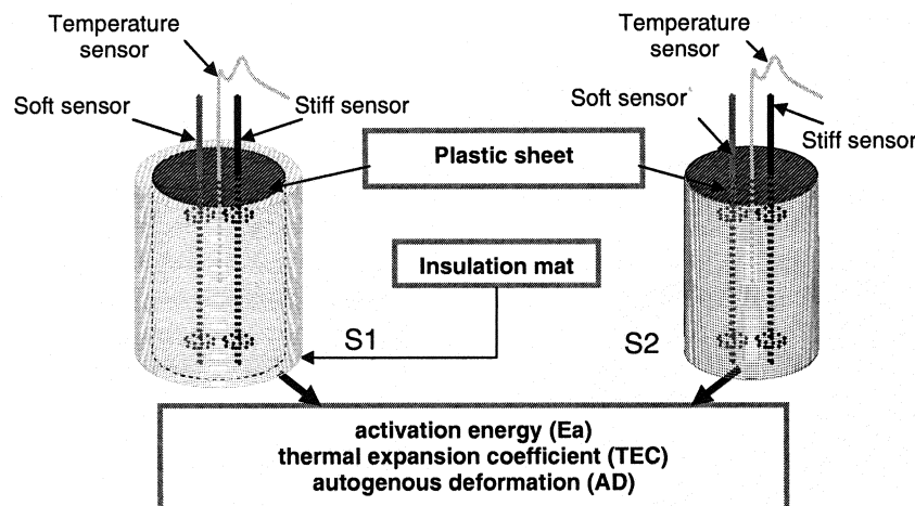
Fig. 1. Separation of effects through differently cured specimens.
