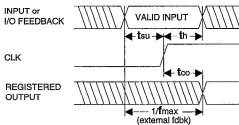
Registered Output
