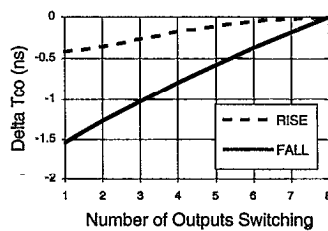
Switching Delta Tco vs # of Outputs Switching
