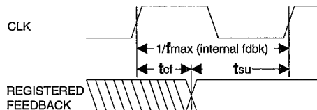
fmax with Feedback
