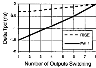
Switching Delta Tpd vs # of Outputs Switching
