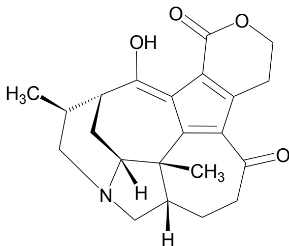
Daphnicyclidin A
