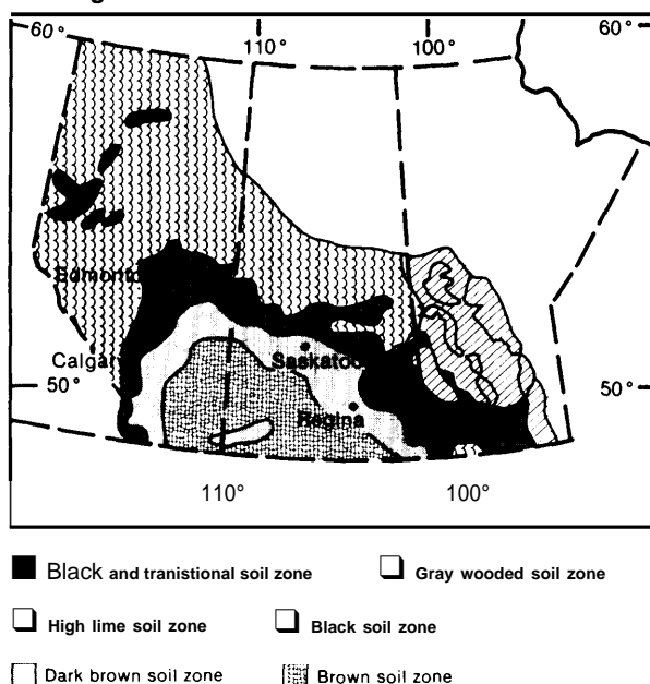
Figure 4.2.—Soil Zones of Western Canada
