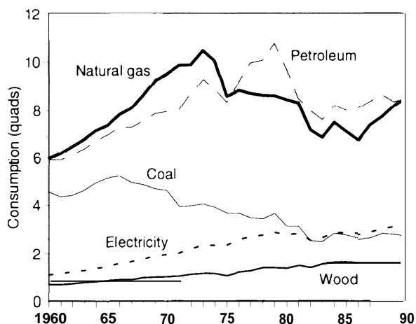
Figure 2-4—Industrial Energy Consumption by Fuel, 1960-90
