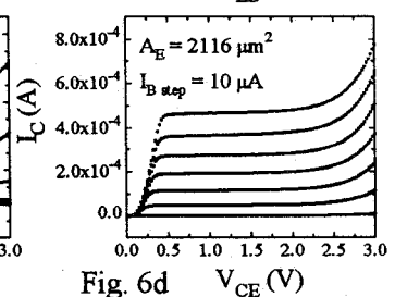
Fig. 6 Transistor curves for devices with As implanted emitters. As grown I_C is from Fig. 3a transistor structure.
