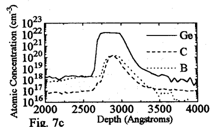
Fig. 7. SIMS of SiGe, SiGeC, and SiGe/SiGeC/SiGe devices with emitters implanted with As and annealed at 755 C.
