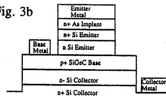
Fig. 3 Device cross sections used to isolate the effects of (a) thermal annealing and (b) emitter implants.
