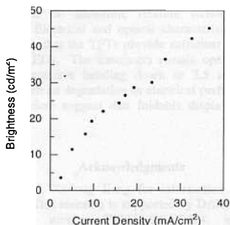
Figure 6. OLED luminance as a function of current through the device.
