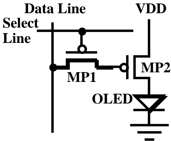
Fig. 1. Two-Transistor AMOLED Pixel.
