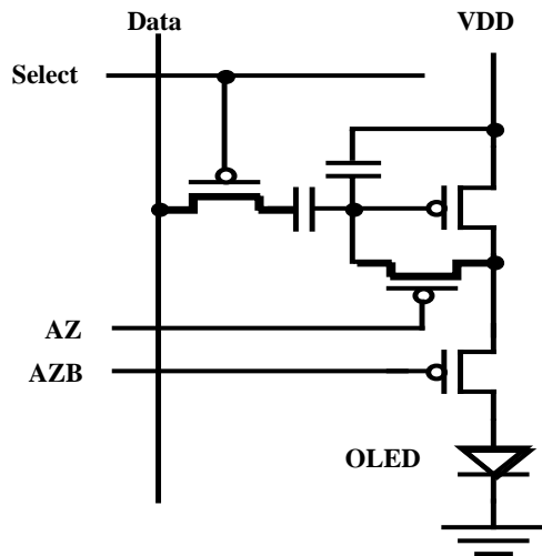
Fig. 3. Schematic of Four-Transistor AMOLED Pixel with Autozero.
