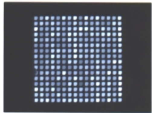
Fig. 2. Luminance non-uniformity of the two-transistor pixel caused by local variations in the transistor output characteristics.
