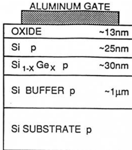
Fig. 3. Sample device structure for a buried layer silicon-germanium capacitor with a thermal oxide insulator. A voltage pulse applied between the gate and the substrate forces the capacitor into deep depletion with the depletion region residing primarily in the Si 1-x Ge x layer.
