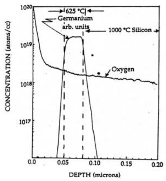
Fig. 2. SIMS profile of oxygen concentration in a multilayer Si 1-x Ge x sample grown with a load-lock.
