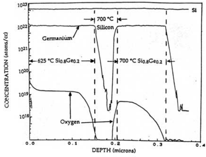
Fig. 1. SIMS profile of oxygen concentration in a multilayer Si 1-x Ge x sample grown without a lock-lock.
