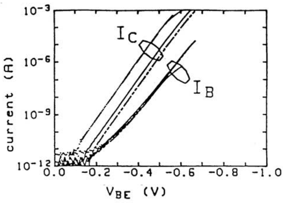
Fig. 6 Room temperature Gummel plots of npn Si/SiGe/Si graded base HBT's with varying base compositions. 0-20% Ge, dot-dash; 7-20% Ge, solid; 13-20%, dashed; and 20% Ge, not graded, dotted.
