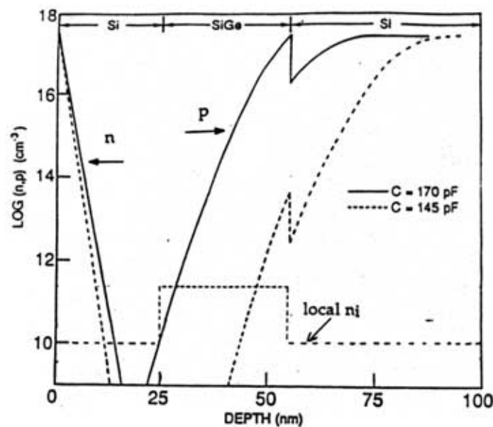
Fig. 4 Logarithm of the carrier profiles as a function of depth into the device for the buried layer Si 1-x Ge x capacitor at two points during its recovery from deep depletion to inversion. For C > 170 pf, the generation in the SiGe is not depressed by high carrier levels. The discontinuity of the hole concentration reflects the discontinuity of the valence band at the Si/Si 1-x Ge x interface.
