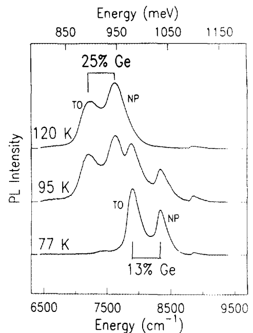
FIG. 5. High-temperature luminescence of the triple well structure of Fig. 4. Note at 95 K and above the excitons thermally hop out of the x = 0.13 wells and are captured by the central x = 0.25 well.
