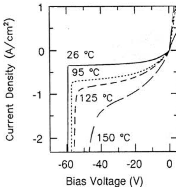
Fig.3 I-V characteristics of a Pt Schottky barrier at different measurement temperatures. The breakdown voltage decreases as temperature increases.
