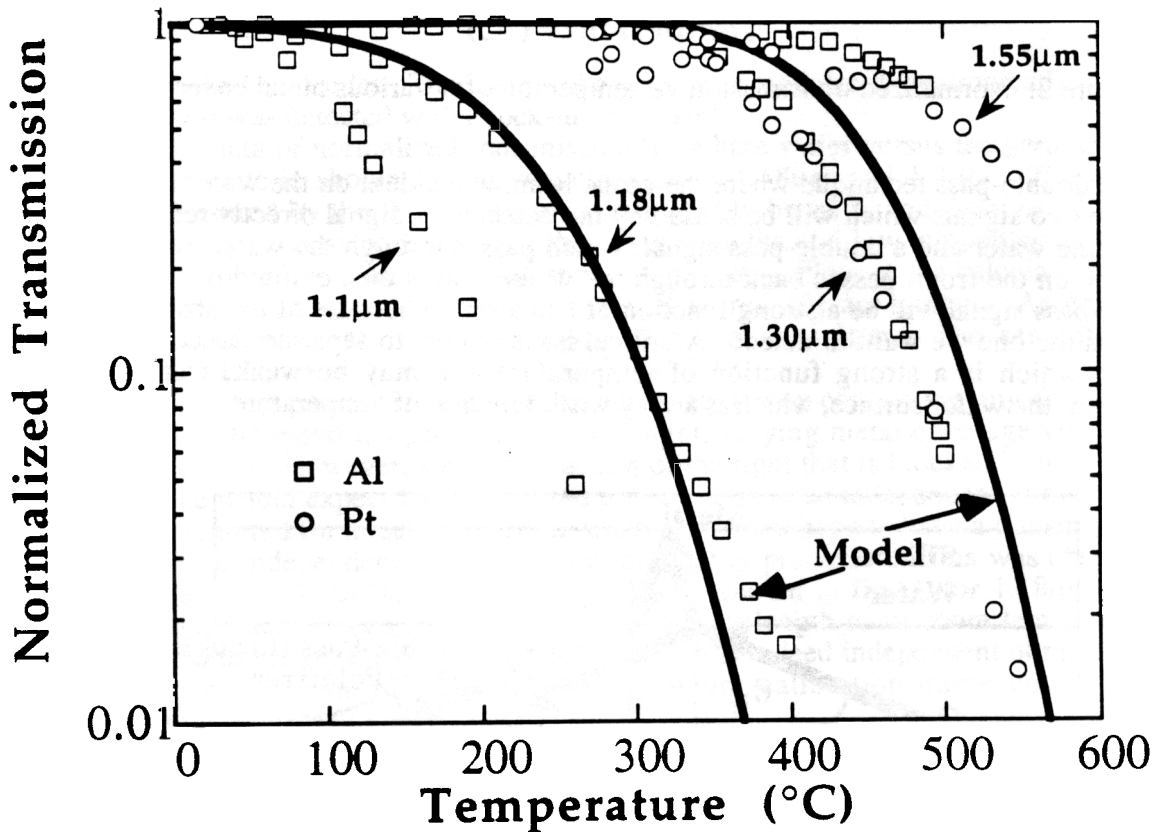
Figure 4: Normalized double-pass transmission data at 1.1, 1.18, 1.3, and 1.55\mu\text{m} vs. temperature and modeling results.
