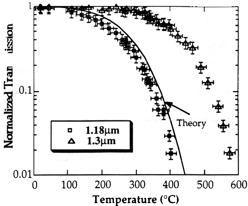
Figure 1: Normalized transmission vs. temperature for 1.18 \mu\text{m} and 1.30 \mu\text{m} .
