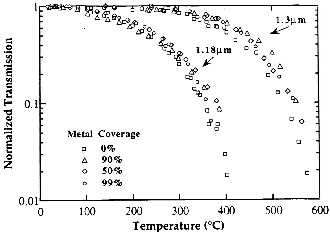
Figure 2: Normalized transmission vs. temperature for various metal coverages.
