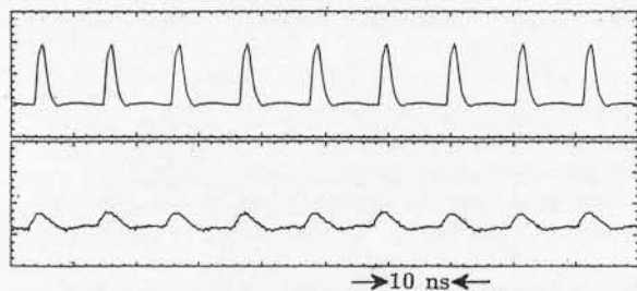
Fig. 5. Switch on of the signal beam at 1.5 \mu\text{m} with a 2-ns recovery time. Both the signal (upper trace) and the control (lower trace) beams are focused to \sim 5\ \mu\text{m} in diameter.
