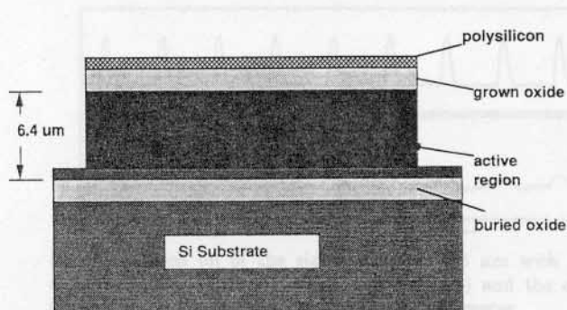
Fig. 1. Cross section of the asymmetric Si Fabry-Perot étalon.
