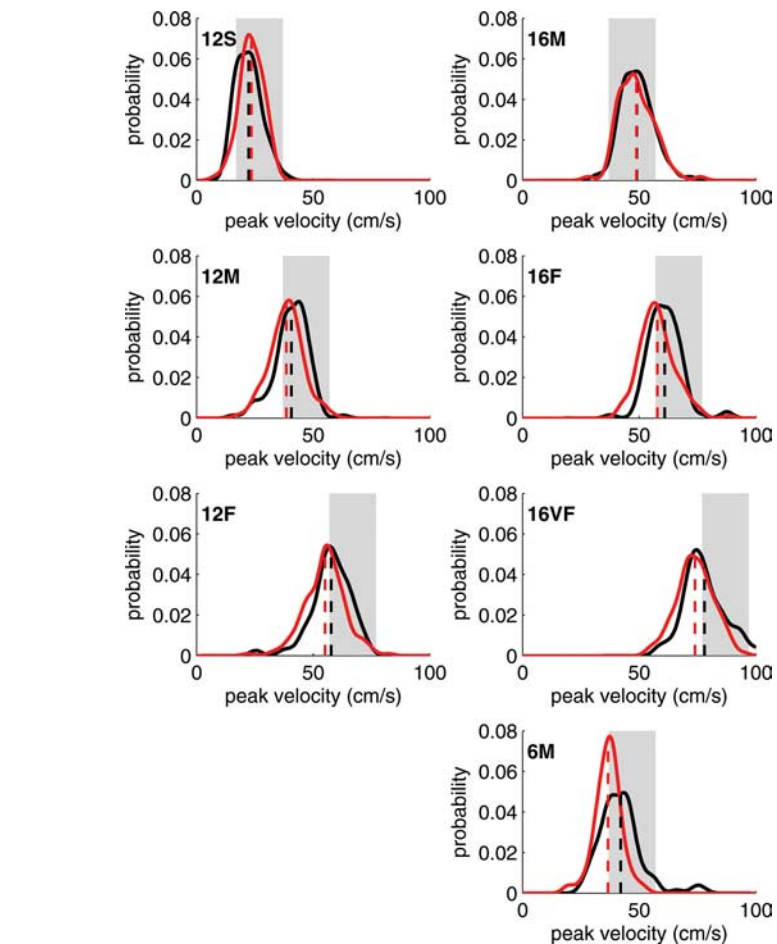
Figure 1. Velocity probability distributions of Parkinson's patients are shifted toward slower movements in all but the easiest conditions. Probability distribution functions for each condition were estimated using kernel density estimation based on all movements (valid and invalid) (see Mazzoni et al., 2007), and normalized [for non-normalized histograms, see Mazzoni et al. (2007), their Fig. 7 ( http://www.jneurosci.org/cgi/content/full/27/27/7105/F7 )]. In red are the estimated distributions for PD patients, in black are those for healthy controls. Shaded areas mark the required range of velocities in each condition [slow (S), 17–37 cm/s; medium (M), 37–57 cm/s; fast (F), 57–77 cm/s; very fast (VF), 77–97 cm/s], and numbers in bold (6, 12, or 16) denote the distance to target in centimeters. Dashed line, Empirical mean. Data are courtesy of Dr. Pietro Mazzoni (Mazzoni et al., 2007)
