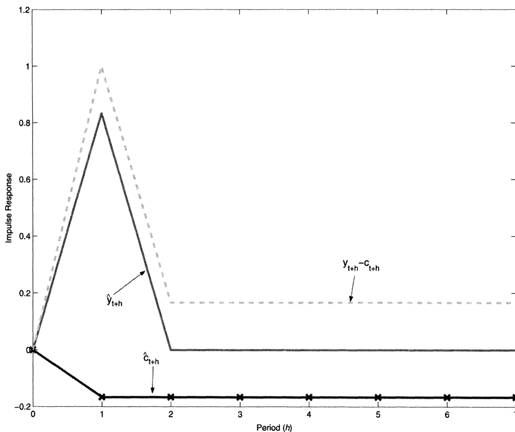
FIGURE 2. IMPULSE RESPONSES OF \hat{y}_{t+h} , \hat{c}_{t+h} , AND y_{t+h} - c_{t+h} TO A SHOCK IN \varepsilon_t
