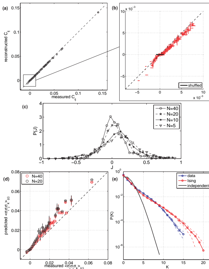
FIG. 1: (a) Precision of the Ising model learned via Eq (3): measured covariance elements are binned on the x-axis and plotted against the corresponding reconstructed covariances on y-axis; vertical error bars denote the deviation within the bin and horizontal error bars denote the bootstrap errors on covariance estimates. (b) Zoom-in for small C_{ij} , with scale bar representing the distribution of covariances from shuffled data. Not shown are the reconstructions of the means, \langle \sigma_i \rangle , which are accurate to better than 1%. (c) Distribution of coupling constants J_{ij} . (d) Measured vs predicted connected three-point correlations for 40 neurons (red) and exact solution for a 20 neuron subset (black). (e) Probability of observing K simultaneous spikes, compared to the failure of the independent model (black line). Dashed lines show error estimates.
