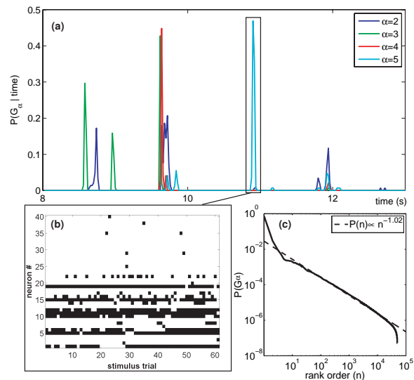
FIG. 3: (a) Probability that the 40 neuron system is found in a configuration within the basin of each nontrivial ground state \mathcal{G}_\alpha , as a function of time during the stimulus movie; P(\mathcal{G}_\alpha | t) = 0.4 means that the retina is in that basin on 40% of the 145 repetitions of the movie. (b) All unique patterns assigned to \mathcal{G}_5 at t = 10.88 - 10.92 s. (c) Zipf plot of the rank ordered frequencies with which the lowest lying 5 \cdot 10^4 stable states are found in the simulated 120 neuron system.
