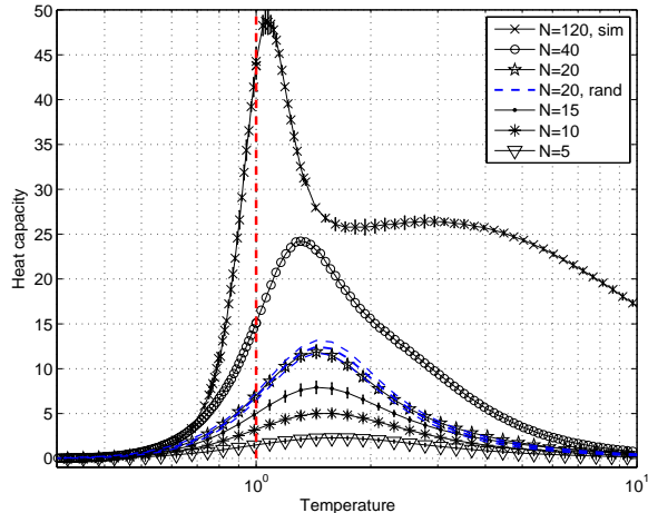
FIG. 2: C(T) for systems of different sizes. Ising models were constructed for 400 subnetworks of size 5, 180 of size 10, 90 of size 15 and 20, 1 full network of size 40 (all from data), and 3 synthetic networks of size 120; vertical error bars are standard deviations across these examples. The mean of the heat capacity curve and the 1 sigma envelope for Ising models of randomized networks are shown in blue dashed lines.
