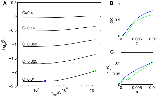
FIG. 8: The dependence of information transmission in the self-activating case on the ratio \gamma_{\max}/C . A) For various choices of C indicated on the plot, the information transmission with the optimal choice with respect to all parameters \theta is shown as a function of \gamma_{\max}/C . Two special systems of interest (blue, green) are chosen for the lowest value of C . B) The mean input/output relation for the blue and green system. The green system has a higher transmission, a steeper activation curve but a smaller dynamic range. C) The effective noise in the input, \sigma_c(c) , for the blue and green systems. The green system is closer to critical at the point where the mean input/output curve has the highest curvature and the noise exhibits a dip.
