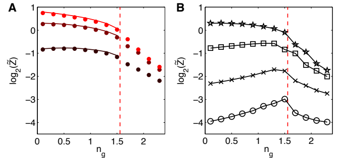
FIG. 9: Crossing the critical line (dashed red) into the bistable region. A) Capacity as a function of n_g at fixed K_g = 0.05 , with the optimal choice of \{n_c, K_c, c_{1/2}\} parameters, for three values of C ( C = 0.1, 1, 10 dark to bright red, respectively). Dots show capacity calculation using the bistable code that can handle multiple branches using Eq (85), solid line uses the monostable integration as in Eq (36). B) Optimal capacity at very high ratios \gamma_{\max}/C = 10^3 for different value of C ( C = 10^{-3}, 10^{-2}, 10^{-1}, 1 : circles, crosses, squares, stars, respectively). The optimum is pushed towards the critical line from the monostable side for \gamma_{\max}/C large and C small. In all cases, information in the bistable regime is smaller than in the monostable regime.
