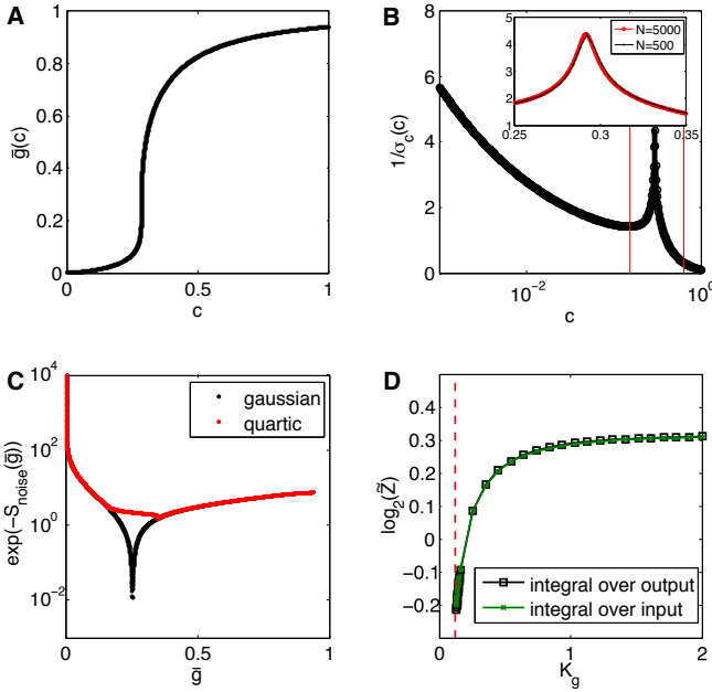
FIG. 3: Computing information transmission close to the critical point. A) An input/output relation \bar{g}(c) for n_g = 2 , C = 1 and K_g = K_g^*(n_g) + 0.004 , showing a self-activating gene with an almost critical value of K_g . B) Noise in the input from Eq (14), which is the integrand in the expression for information in Eq (36), shows an incipient divergence between red vertical bars. Inset: zoom-in of the peak shows that it can be sampled well by increasing the number of bins. Different plot symbols indicate domain discretization into 500 (black dots) and 5000 (red circles) bins. At the critical point the divergence is hard to control numerically. C) An alternative way of computing the same information, by integrating in the output domain as in Eq (69). Shown is the integrand in the gaussian noise approximation [black, S_2(\bar{g}) from Eq (66)] and with quartic corrections [red, S_4(\bar{g}) from Eq (67)]. At the critical point higher order corrections regularize the integrand, while away from the critical point the integrand smoothly joins with the gaussian approximation. This approach is stable numerically both away from and in the critical regime. D) Information I = \log_2 \bar{Z} as a function of K_g for n_g = 2 . Critical K_g^* = 1/8 is denoted by a dashed red line. Integration across \bar{g} in the output domain with quartic corrections (squares) agrees well with the integration across c in the input domain (crosses) away from K_g^* , but also smoothly extends to the critical K_g^* . This is a cut across the capacity plane in Fig 4A (denoted by a dashed yellow line) for C = 1 .
