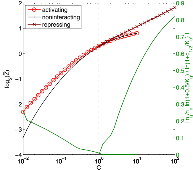
FIG. 6: Information transmission in a system where all parameters \theta are optimized as a function of the maximal input concentration C . The self-interacting system (red) allows for an arbitrary MWC-like regulatory function [Eq (38)] with parameters \theta = \{c_{1/2}, n_c, K_c, n_g, K_g\} . The noninteracting system (black) only has the MWC parameters n_c, K_c and the leak L (see Ref [7]) which can be reexpressed in terms of c_{1/2} . Bright red line with circles shows self-activating solutions which are optimal for C < 1 , while dark red line with crosses shows self-repressing solutions, optimal for C > 1 . Plotted on the secondary vertical axis in green is the ratio between the self-interacting contribution to F , and the input contribution to F in the expression for the MWC regulatory function [Eq (38)]. For C \sim 1 where the interacting and non-interacting solution join, this term falls to 0, as expected.
