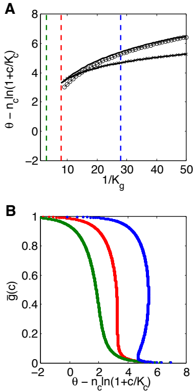
FIG. 2: Monostable (green), critical (red) and bistable (blue) behavior of the self-activating gene for n_g = 2 . A) The phase diagram as a function of K_g and the input-dependent term. In the region between the black solid lines two solutions \bar{g}_{1,2} exist for every value of the input c (y-axis). The corresponding critical value is at K_g^* = 1/8 (cusp of the black solid lines). Circles and crosses represent analytical approximations to the exact boundary of the bistable region for n_g = 2 and large 1/K_g (see text). For three choices of K_g denoted by vertical dashed lines, the input / output relations \bar{g}(c) are plotted in B. B) The critical solution (red) has an infinite total derivative \bar{g}'(c) at \theta - n_c \ln(1+c/K_c) = 3.29 , \bar{g} = 0.25 . The bistable system (blue) has three solutions, two stable and one unstable, for a range of inputs that can be read out from the plot in A.
