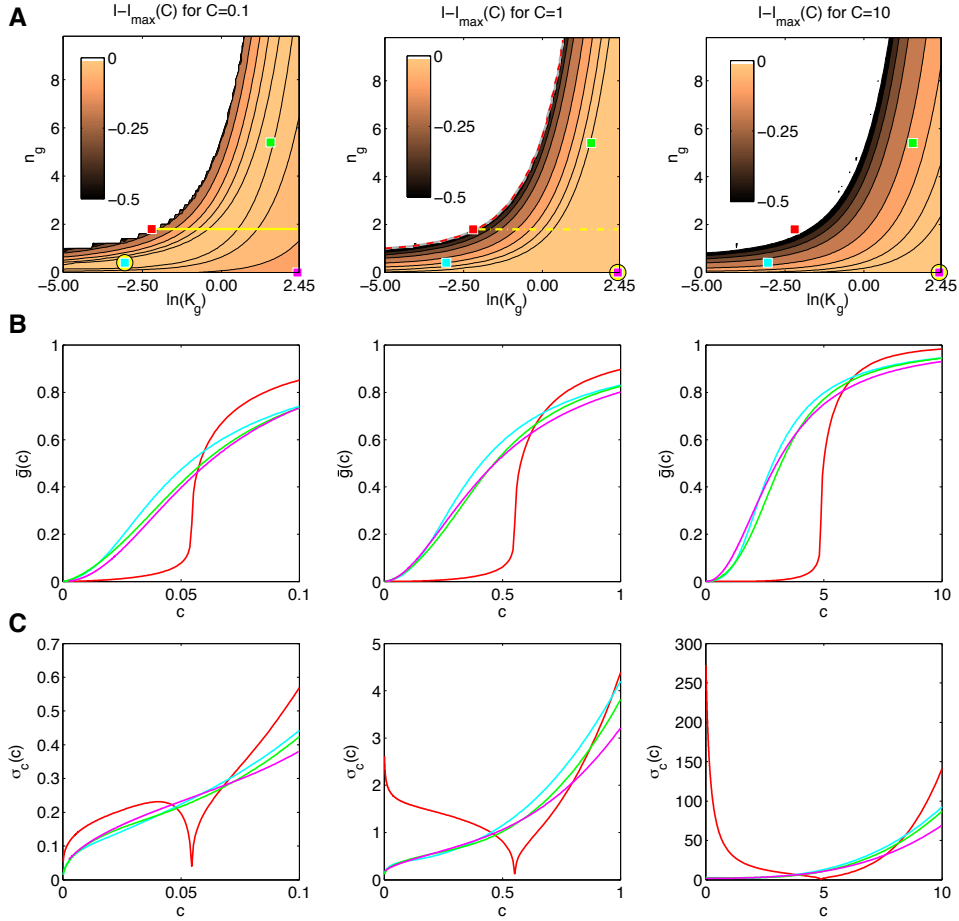
FIG. 4: Information transmission as a function of self-activating parameters \{n_g, K_g\} for three values of C ; C = 0.1 (left column), C = 1 (middle column), C = 10 (right column). For each value of \{n_g, K_g\} the three remaining parameters \{c_{1/2}, n_c, K_c\} are optimized to maximize information. A ) The capacity planes showing the decrease in capacity in bits (colormap) from the maximal value achieved for an optimal choice of all parameters; the optimal set of parameters is denoted by a colored square on a yellow circle. The white upper left region of each capacity plane corresponds to the bistable region. For low C = 0.1 the maximum is achieved in the interior of the domain (cyan square), while for C = 1, 10 n_g is driven to 0 (magenta squares), corresponding to the non-self-interacting solution. Red square represents an example critical system at n_g = 2 and the green square represents a self-interacting system with a high value for n_g . The yellow dashed line in C = 1 plane represents a cut shown in detail in Fig 3D. The yellow solid line in C = 0.1 plane represents a cut shown in detail in Fig 5A. The red dashed boundary of the critical region in C = 1 plane is analyzed in detail in Figs 5B, 5C. B ) Input/output relations for 4 example systems denoted by colored squares in A. Despite substantially different values for \{n_g, K_g\} , the optimization of remaining parameters makes the input/output curves look very similar to the optimal solutions, except for the critical (red) curves. C ) The effective input noise \sigma_c(c) for the selected systems.
