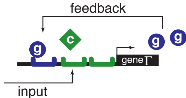
FIG. 1: A schematic diagram of a self-regulating gene. The gene \Gamma is depicted by a thick black line and a promoter start signal. Gene products g denoted as blue circles can bind to the regulatory sites (one in this example) that control the expression of \Gamma . Direct control over the expression of \Gamma is exerted by molecules of the transcription factor c (green diamonds, two binding sites).
