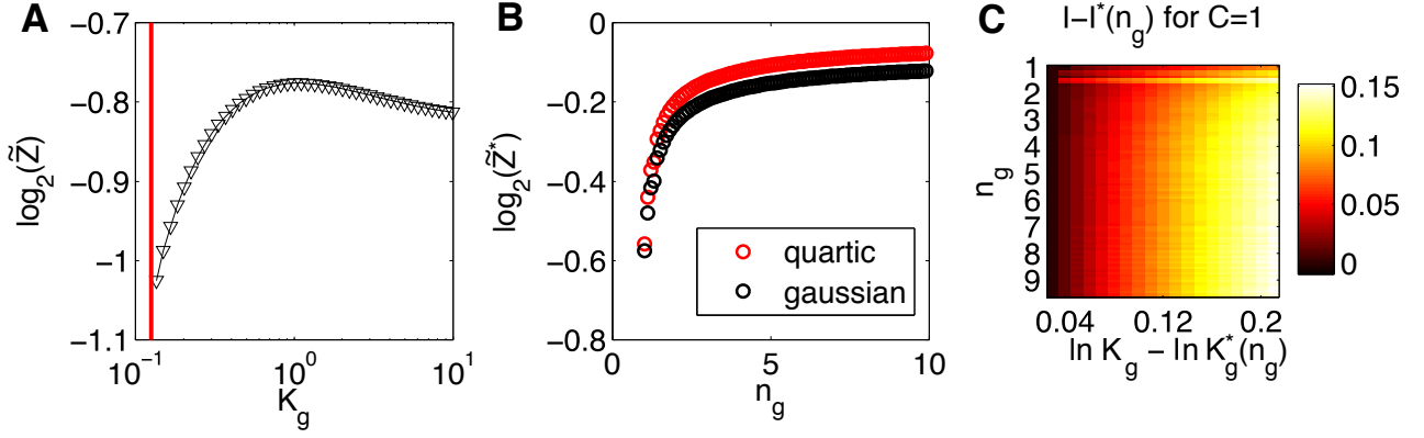
FIG. 5: Information transmission close to the critical line. A) A detailed scan of information for C = 0.1 as the function of K_g for n_g = 2 and optimal choice for \theta_c for every K_g exhibits a peak for a nontrivial value of K_g . B) The information transmission along the critical line for C = 1 as a function of n_g indicates that while including quartic corrections is important, the information at the critical line does not exhibit any large jumps (not shown). C) A detailed scan of capacity close to the critical line for C = 1 as a function of n_g (vertical axis). Shown in color is the increase in information in bits compared to the value very close to the critical I^*(n_g) , as a function of the distance in K_g from the critical value (horizontal axis). Across the range of n_g , going from the critical axis into the monostable domain increases the information.
