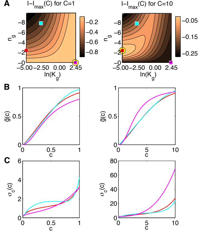
FIG. 7: Information transmission as a function of self-repressing parameters \{n_g, K_g\} for C = 1 (left column) and C = 10 (right column); plot conventions are the same as in Fig 4. A ) The capacity decrease from the maximum value (achieved at the parameter choice indicated by a yellow circle) as a function of \{n_g, K_g\} . The maximum information transmission is achieved for a non-interacting case (magenta), for C = 1 . In contrast, for C = 10 , there is a non-trivial optimum for small values of K_g and n_g \approx -2.5 (red). B ) The mean input/output solutions for three example systems from A (red, magenta, cyan). C ) The effective noise in the input, \sigma_c(c) , for example solutions in A.
