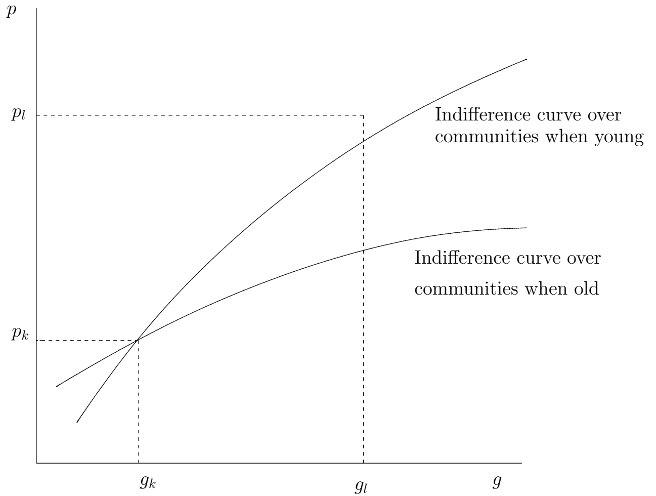
Figure 4: Indifference Curves by Cohort
