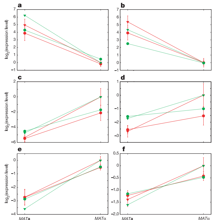
Figure 2 | Example transcripts showing genetic interaction between MAT and GPA1 . Each panel represents one transcript: a , YFL026W/STE2 ; b , YIL015W/BAR1 ; c , YJR004C/SAG1 ; d , YGL090W/LIF1 ; e , YCR040W/MAT \alpha 1; f , YCR039C/MAT \alpha 2. Each red point represents the mean expression level over segregants with one genotype, normalized by the mean over segregants inheriting the BY allele at both loci; red error bars represent standard deviations among segregants with the respective genotype. Each green point represents the expression level in one engineered strain, normalized by the level in the engineered strain with the BY allele at both loci. Strain mating type is indicated on the x axis ( MAT a is the RM allele, MAT \alpha is the BY allele). Triangles and circles represent strains carrying the BY and RM alleles of GPA1 , respectively.
