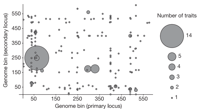
Figure 1 | Genome distribution of QTL pairs detected by the two-stage linkage search. On each axis the genome is divided into 611 bins of 20 kilobases each, shown in chromosomal order. The set of transcripts mapping to QTLs in each pair of bins in the two-stage analysis is represented as a circle, with the width proportional to the number of such co-linking transcripts (a scale is shown at the right); circles are centred on the corresponding bins. The largest circle represents the MAT – GPA1 locus pair.
