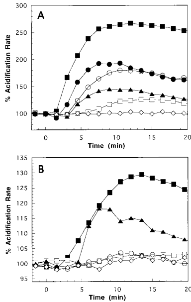
Figure 2. Cytosensor Analysis of T Cell Activation by MCC/IE k Oligomers
