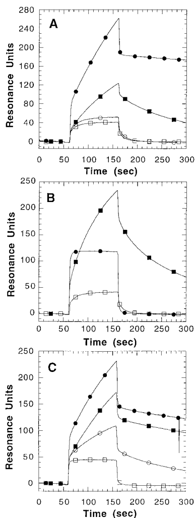
Figure 1. BIAcore Binding Analysis of IE k Oligomers to the 2B4 TCR (A) MCC/IE k complexes were passed over 2B4 TCR coupled to the sensor chip. Shown is the binding of MCC/IE k -only (open squares), MCC/IE k monomer (open circles), dimer (solid squares) at 33 µg/ml, and tetramer (solid circles) at 72 µg/ml. (B) Shown is the binding of MCC/IE k -only (33 µg/ml) (open squares), MCC(102S)/IE k (200 µg/ml) (solid circles), and MCC(102S)/IE k tetramer (100 µg/ml) (solid squares). (C) Shown is the binding of the mixed oligomers containing MCC(99A)/IE k in the residual biotin binding sites. Binding was performed at 72 µg/ml monomer (open squares), dimer (open circles), trimer (solid squares), and tetramer (solid circles). Dissociation rates appear faster in (C) because the TCR surface is only half as dense as in (A) and (B). In (A) and (B), concentrations refer to the amount of MCC/IE k but in (C) they refer to the amount of total IE k [MCC and MCC(99A)]. No binding was observed with streptavidin only.
