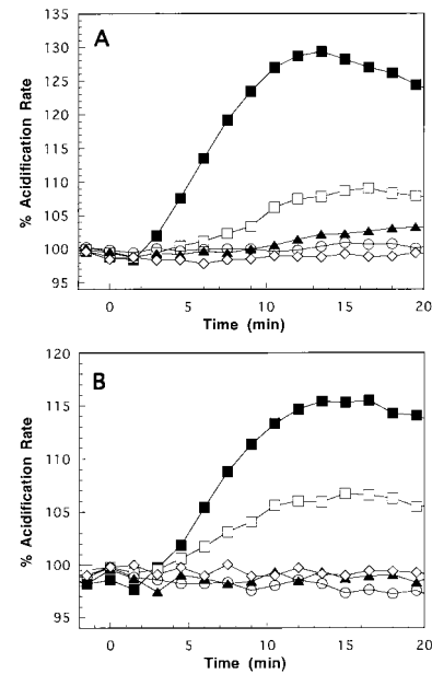
Figure 3. Cytosensor Analysis of T Cell Activation by Mixed Oligomers
