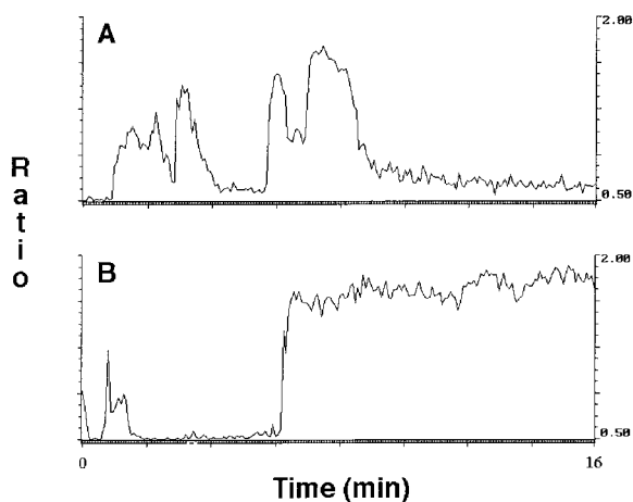
Figure 4. Single Cell Calcium Flux of 5CC7 T Cells (A) Shown is a representative trace of calcium fluctuations in a 5C.C7 T cell at 37°C treated with MCC/IE k tetramer at a concentration of 250 µg/ml. (B) Shown for comparison is a typical calcium response to stimulation by MCC peptide presented on CHO cells transfected with IE k at 25°C as described in Wülfing et al. (1997). At 25°C, the response to tetramer was generally more lagged than that shown at 37°C.
