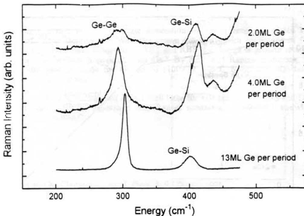
Figure 4. Raman scattering spectra of Ge/Si superlattices.
