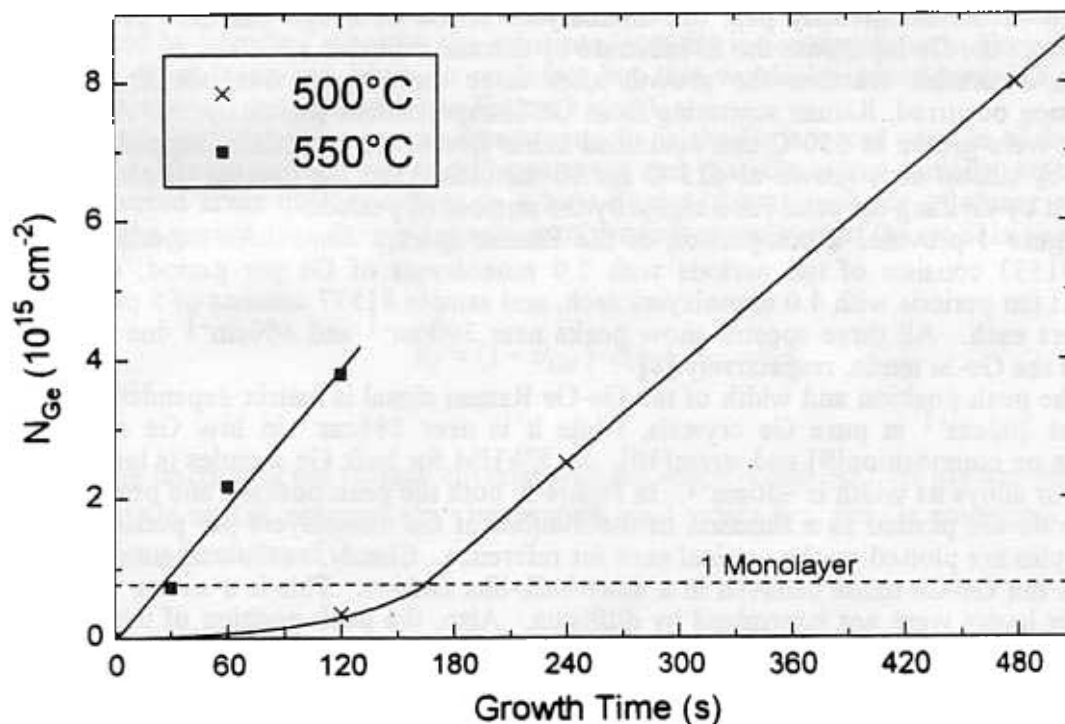
Figure 1. Ge coverage on Si as a function of growth time at 500°C and 550°C
