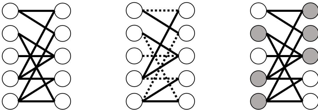
(a) An example of a bipartite graph
