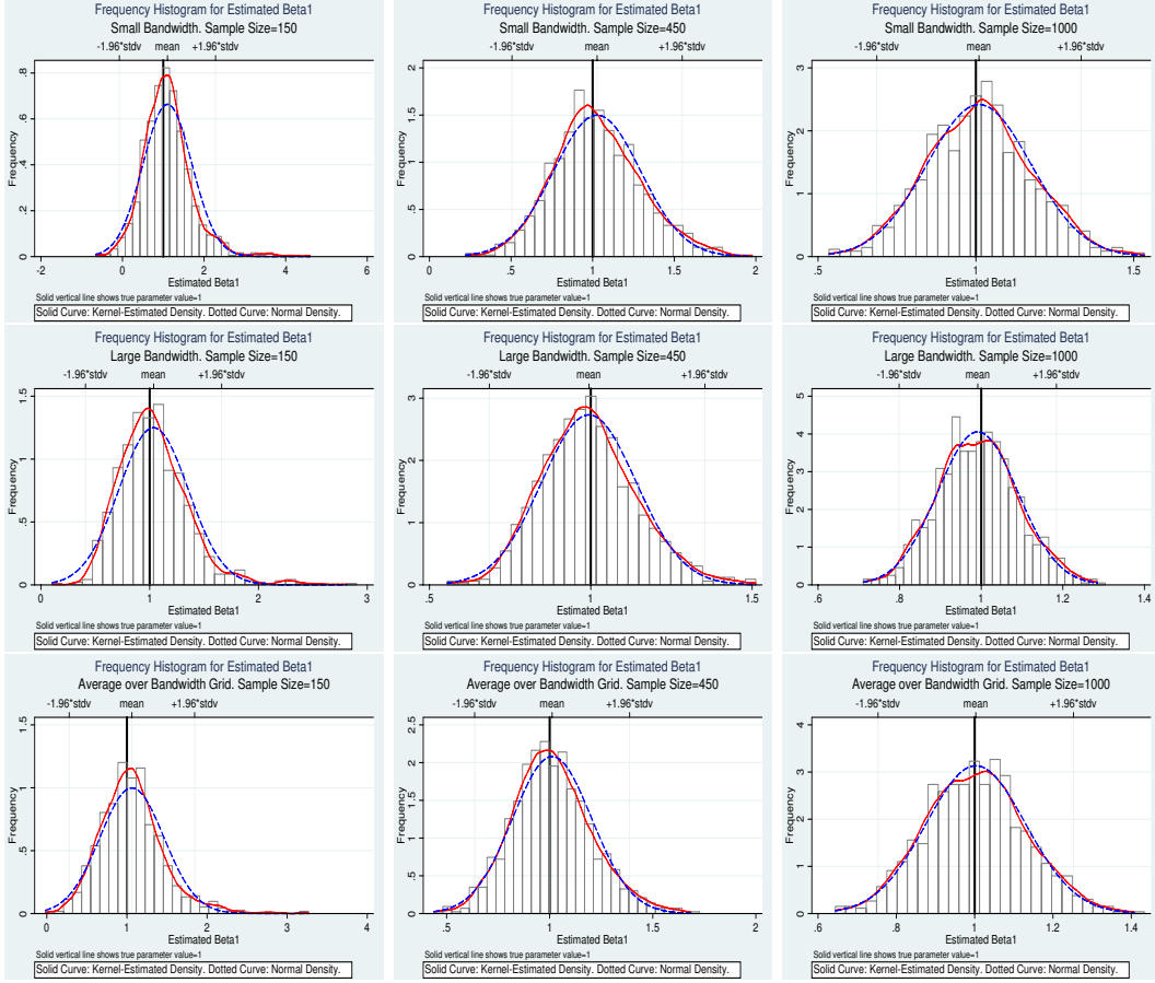
Figure 1: Histogram and Densities for Simulated Estimates of \beta_1 . Rows summarize results for \hat{\beta}_1^I , \hat{\beta}_1^{II} and \hat{\beta}_1^{III} respectively. Columns summarize results for N = 150 , N = 450 and N = 1000 respectively.
