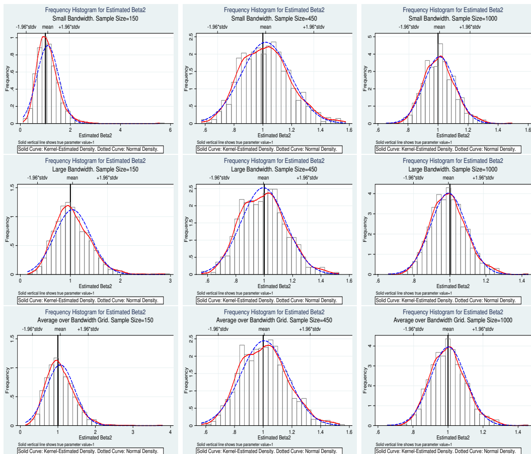
Figure 2: Histogram and Densities for Simulated Estimates of \beta_2 . Rows summarize results for \hat{\beta}_2^I , \hat{\beta}_2^{II} and \hat{\beta}_2^{III} respectively. Columns summarize results for N = 150 , N = 450 and N = 1000 respectively.
