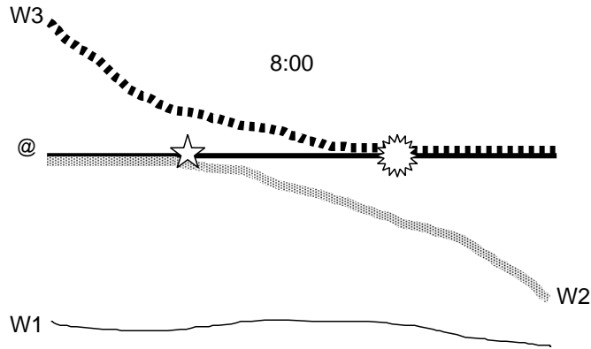
Figure 1: Comparison of three no-crack worlds. The straight solid line labeled “@” represents history in the actual world. W_1 (the thin solid line) contains no violations of actual law, and so differs from the actual world at all times. W_2 (the shaded line) matches actual history until shortly before 8:00, at which time a small divergence miracle (marked by a star) occurs. Thereafter history in W_2 diverges from actual history. W_3 (the dotted line) differs from actual history up until shortly after 8:00, at which time a convergence miracle occurs (marked by a many-pointed star). Thereafter history in W_3 perfectly matches actual history.
