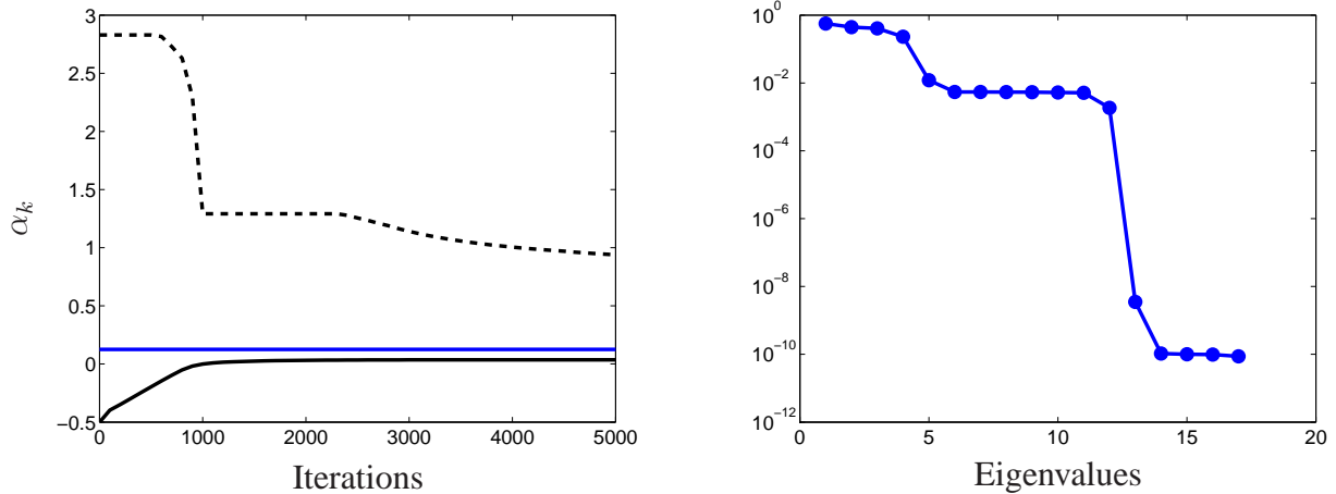
Figure 4: Complexity. Left: Primal and dual bounds on the optimal solution (computed using interior point methods) using the algorithm of Section 5 on a small Gaussian matrix. Right: Screenshot of the optimal solution to (9) for a small Gaussian matrix (obtained by interior point methods with a target precision of 10^{-8} ).
