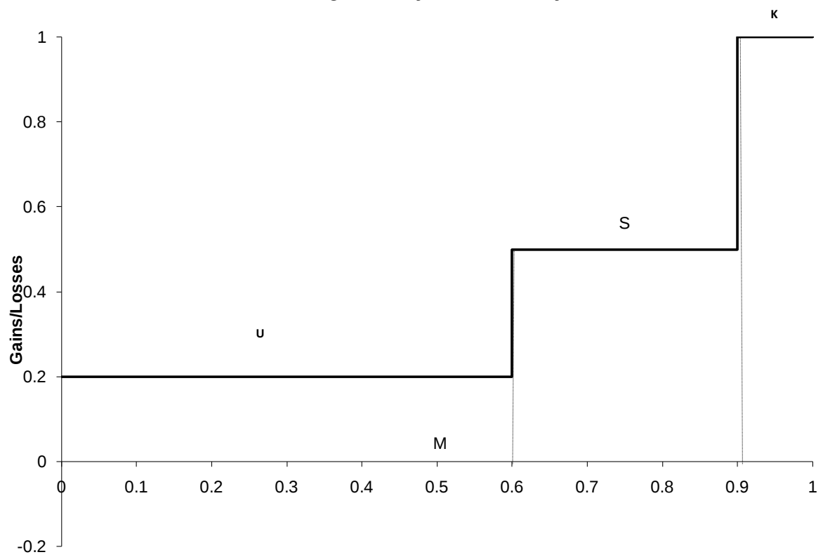
Figure 1. Stylized Economy
