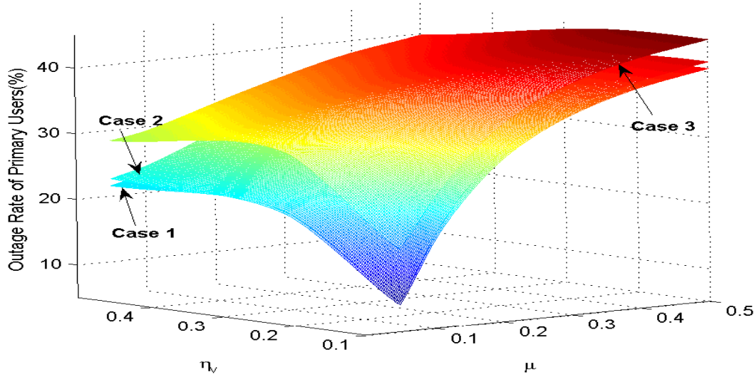
Fig. 6. Comparative analysis of the mean outage rate obtained by N = 15 primary network users with differing degrees of variation in the stochastic link gains and the measurement noise. Three distinct cases were considered: Case 1 consisted of no secondary network, Case 2 involved M = 5 secondary users with Kalman filters, and Case 3 consisted of M = 5 secondary users without estimators. Each secondary user was assigned \rho = 200 : i \in S = \{16, 17, \dots, 20\} by the LSS.
