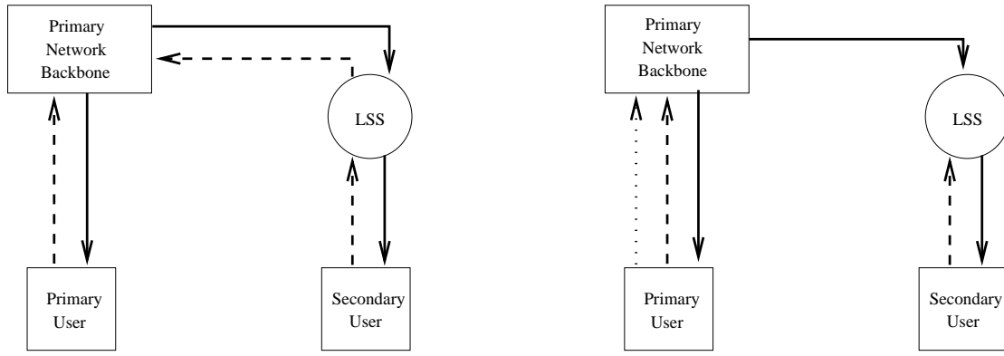
Fig. 2. Two architectures for admission control in a power-controlled cognitive radio network. The solid lines correspond to admission-related commands, the dashed lines indicate admission requests, and the dotted line represents a distress signal.
