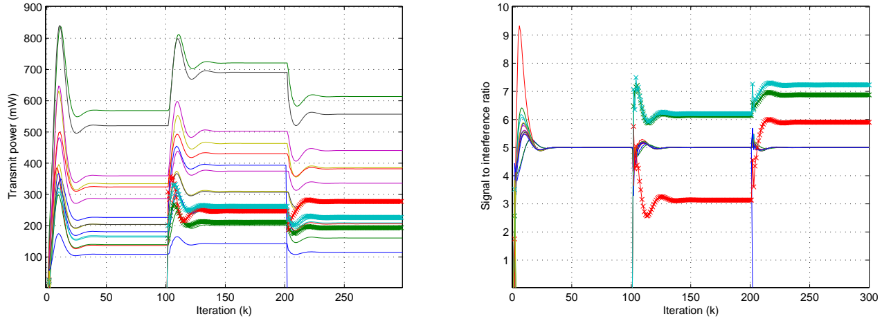
Fig. 3. Dynamics of the transmit power and SIR of the primary and secondary users with a DPCPC policy. The solid lines correspond to the primary users while the thick lines correspond to the secondary users. A target SIR of \text{SIR}_i^{\text{tar}} = 5 was specified for each primary user. The network consisted of N = 15 primary users during 0 < k \leq 100 , N = 15 primary users and M = 3 secondary users for 100 < k \leq 200 , and N = 14 primary users and M = 3 secondary users for 200 < k \leq 300 . The secondary users were assigned \rho_i = 200 : i \in S by the LSS upon their entrance into the network at k = 100 .
