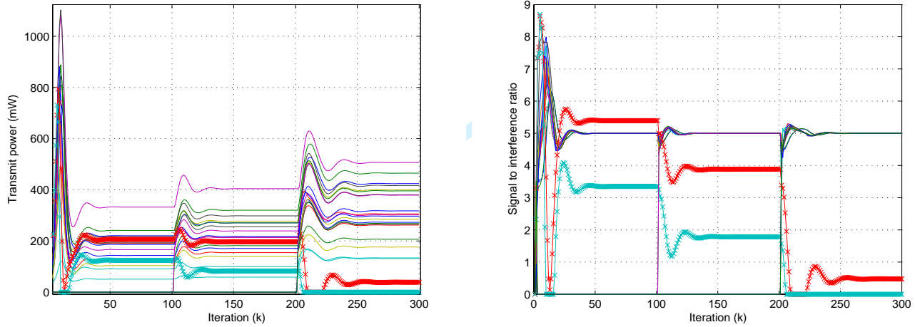
Fig. 4. Dynamics of the transmit power and SIR of the primary and secondary users with a DPCPC policy. The solid lines correspond to the primary users while the thick lines correspond to the secondary users. A target SIR of \text{SIR}_i^{\text{tar}} = 5 was specified for each primary user. The network consisted of N = 15 primary users and M = 2 secondary users during 0 < k \leq 100 , N = 17 primary users and M = 2 secondary users for 100 < k \leq 200 , and N = 21 primary users and M = 2 secondary users for 200 < k \leq 300 . The secondary users were assigned \rho_i = 200 : i \in S by the LSS upon their entrance into the network at k = 0 .
