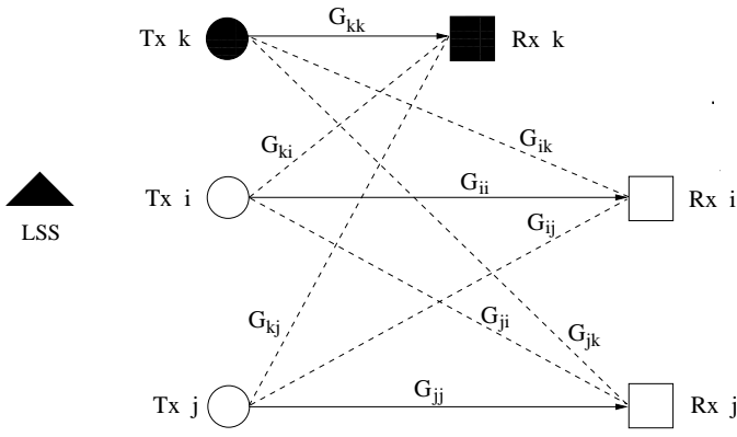
Fig. 1. Model of a cognitive network with transmitter and receiver pairs i and j constituting two primary users, and transmitter and receiver pair k constituting a secondary user. Each link gain is written above the corresponding link with the solid lines denoting intended transmissions and the dashed lines denoting unintended interference among a set of users accessing the spectrum.
