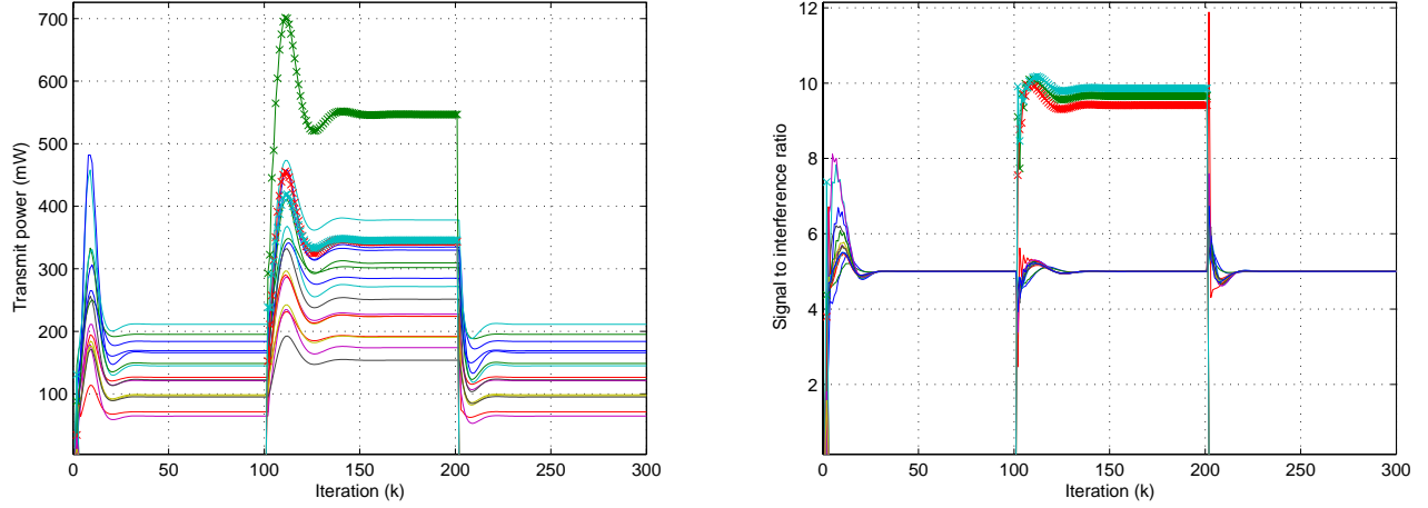
Fig. 5. Dynamics of the transmit power and SIR of the primary and secondary users with a DPCPC policy. The solid lines correspond to the primary users while the thick lines correspond to the secondary users. A target SIR of \text{SIR}^{\text{tar}} = 5 was specified for each primary user. The network consisted of N = 15 primary users during 0 < k \leq 100 , N = 15 primary users and M = 3 secondary users for 100 < k \leq 200 , and N = 15 primary users for 200 < k \leq 300 . The secondary users were assigned \rho_i = 20 : i \in S by the LSS upon their entrance into the network at k = 100 , and assigned \rho = 10^4 : i \in S for k > 200 .
