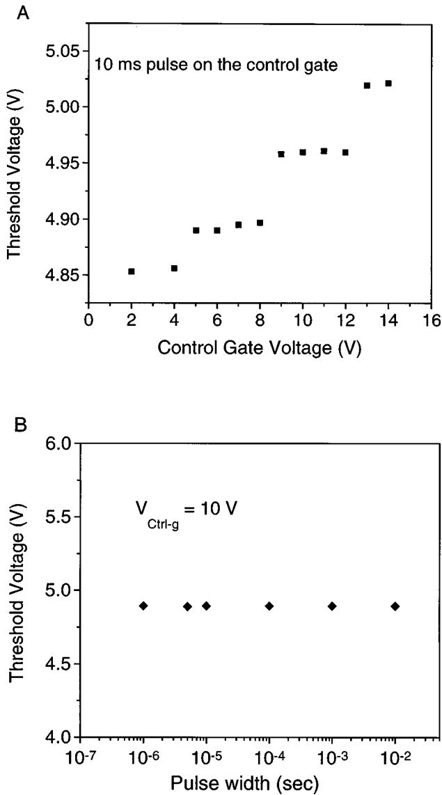
FIG. 5. Threshold voltage of the device as a function of (A) the charging voltage on the control gate, showing a staircase relation with an interval of ~4 V; and (B) as a function of the charging time while the charging voltage pulse is fixed at 10 V, indicating a self-limited process.
