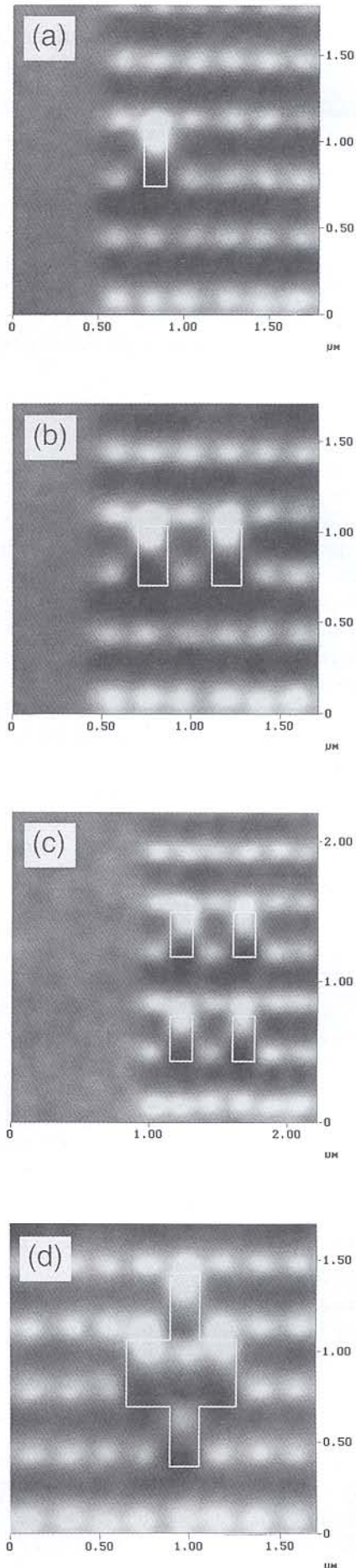
Fig. 3. MFM images of written patterns in the optimum QMD.
