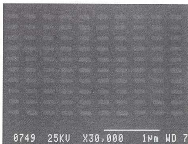
Fig. 1. SEM image of bars in a QMD with density of 10 Gbits/in 2 , a bar thickness of 2 nm(Cr)/10 nm(Co)/5 nm(Cr), a bar size of 200 nm by 60 nm, and a bar spacing of 130 nm.
