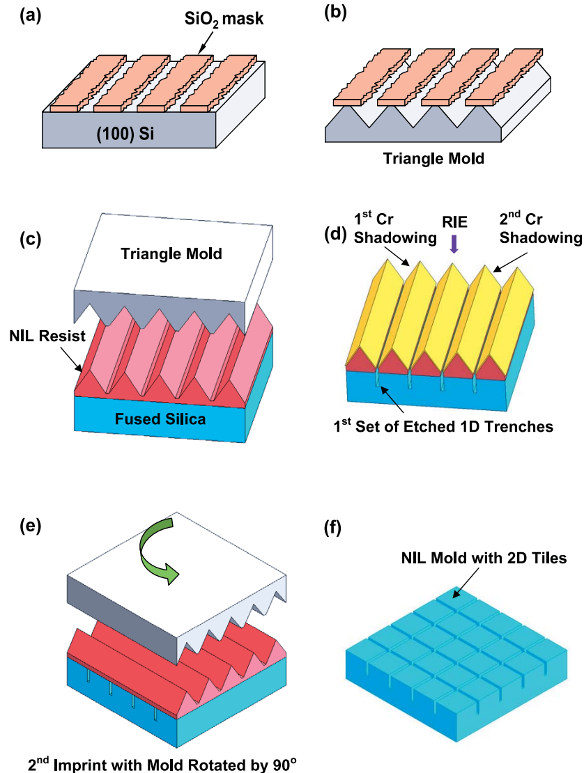
Figure 3. Fabrication of wafer-scale 2D nanotile array mold with sub-10 nm gap. (a) A 200 nm pitch \text{SiO}_2 gratings are patterned on a (100) Si substrate using a grating mold with square profile generated by interference lithography; (b) a KOH-based anisotropic wet etching of the (100) Si substrate creates an imprint mold with a triangle profile and nearly atomically smooth surface; (c) the triangle mold is used to imprint a resist; (d) Cr is shadow evaporated in two well-controlled opposite glancing angles, creating a narrow gap between Cr lines, followed by RIE of the resist residual layer and the \text{SiO}_2/\text{Si} substrate with Cr as the mask; (e) after the removal of Cr and resist in the first imprint cycle, repeat the imprinting (with a triangle mold having the grating oriented 90^\circ from the first imprinted grating), double shadow evaporations of Cr, etching of \text{SiO}_2 , and the final removal of Cr and resist, (e) completing the mold bearing 2D grid pattern.
