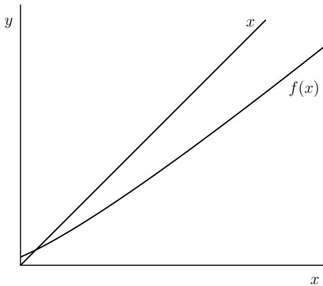
Figure 1: The function y = f(x) for \beta = 0.5 , together with y = x .
