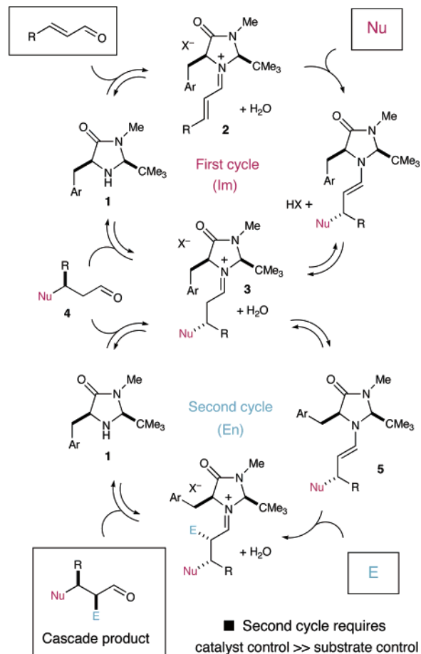
Scheme 1. Cascade Catalysis: Merged Iminium–Enamine Activation
