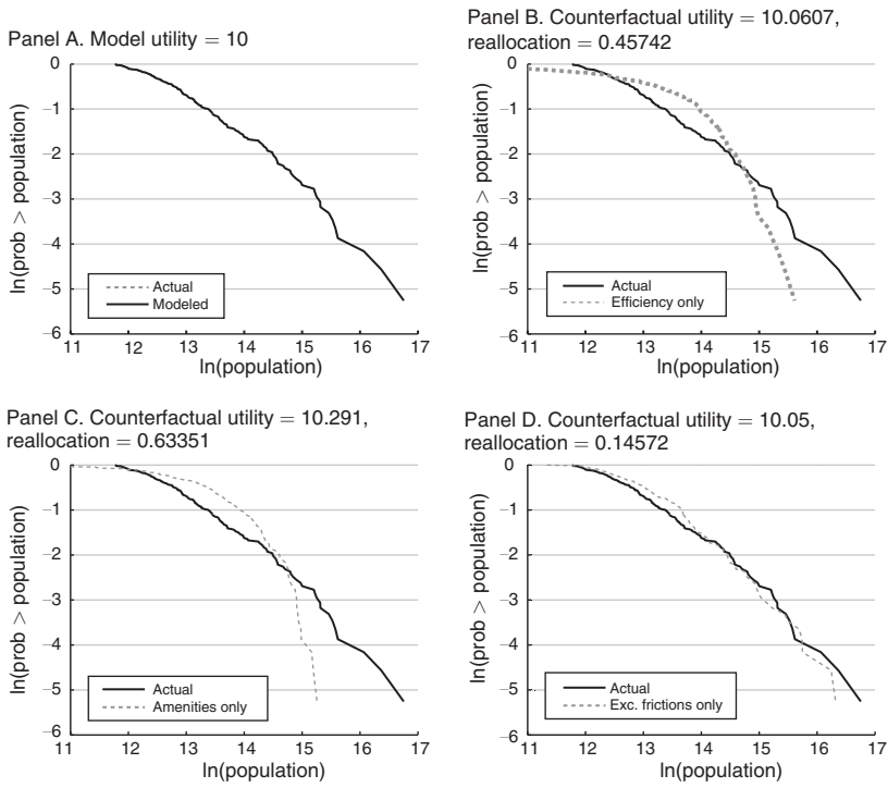
FIGURE 3. COUNTERFACTUALS WITH DIFFERENCES IN ONLY ONE CITY CHARACTERISTIC, \kappa = 0.002
