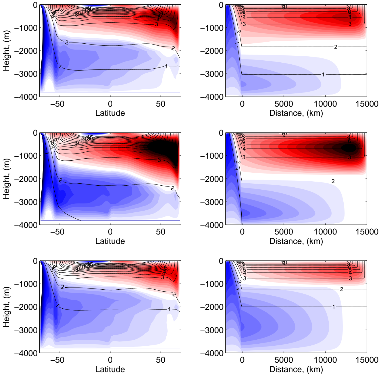
FIG. 9. Zonally-averaged sections of residual circulation ( S_v , blue/red) and temperature ( ^{\circ}\text{C} , black lines) from the GCM simulations (left column) and theory (right column) for the control experiment with \kappa_v = 2 \times 10^{-5} \text{ m}^2 \text{ s}^{-1} and \tau = 0.2 \text{ N m}^{-2} (top row), an enhanced mixing experiment with \kappa_v = 5 \times 10^{-5} \text{ m}^2 \text{ s}^{-1} (middle row), and a reduced Southern Ocean wind experiment with \tau = 0.1 \text{ N m}^{-2} (bottom row).
