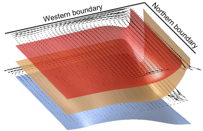
FIG. 6. Three isopycnal surfaces (color) and horizontal flows (black arrows) in the Northern Hemisphere from idealized GCM simulation.
