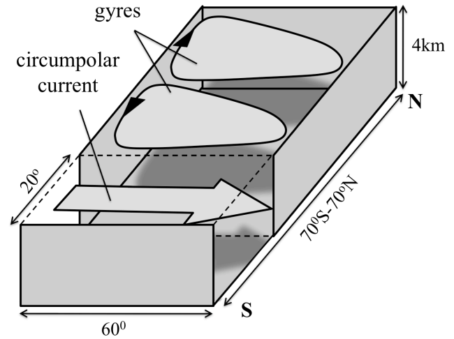
FIG. 3. Schematic of the domain used in idealized simulation. The domain consists of a rectangular basin that connects to a circumpolar full-depth channel at its southern boundary.
