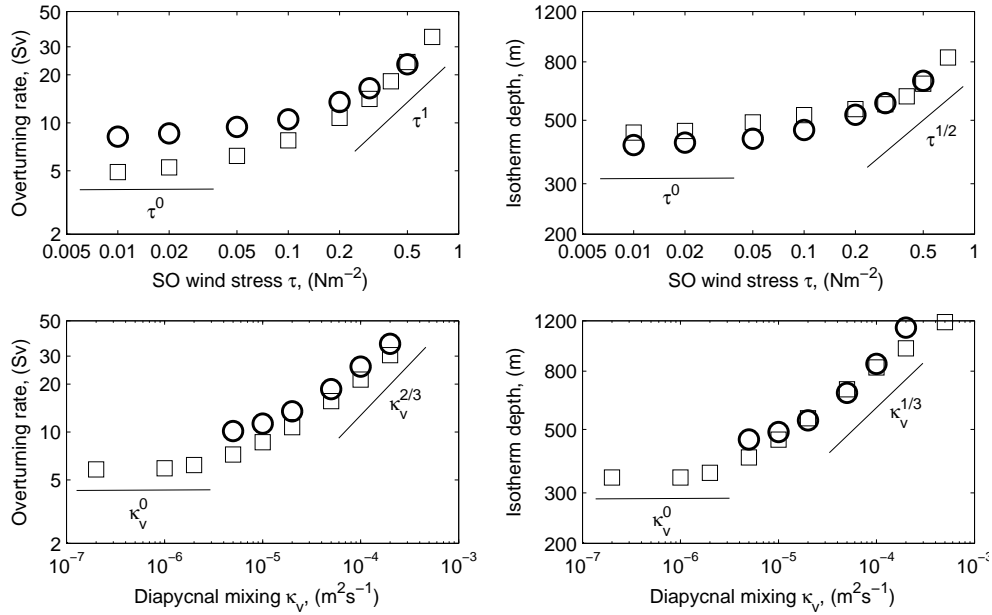
FIG. 11. Rate of the overturning circulation (Sv, left panels) and depth scale of stratification (meters, right panels) as a function of the Southern Ocean wind stress (upper panels) and diapycnal diffusivity (lower panels) estimated from the idealized GCM simulation (circle) and theory (squares).
