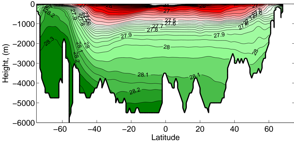
FIG. 1. Meridional section of neutral density ( \text{kg s}^{-3} ) in the Atlantic Ocean at 25^\circ \text{W} from World Ocean Circulation Experiment (WOCE).
