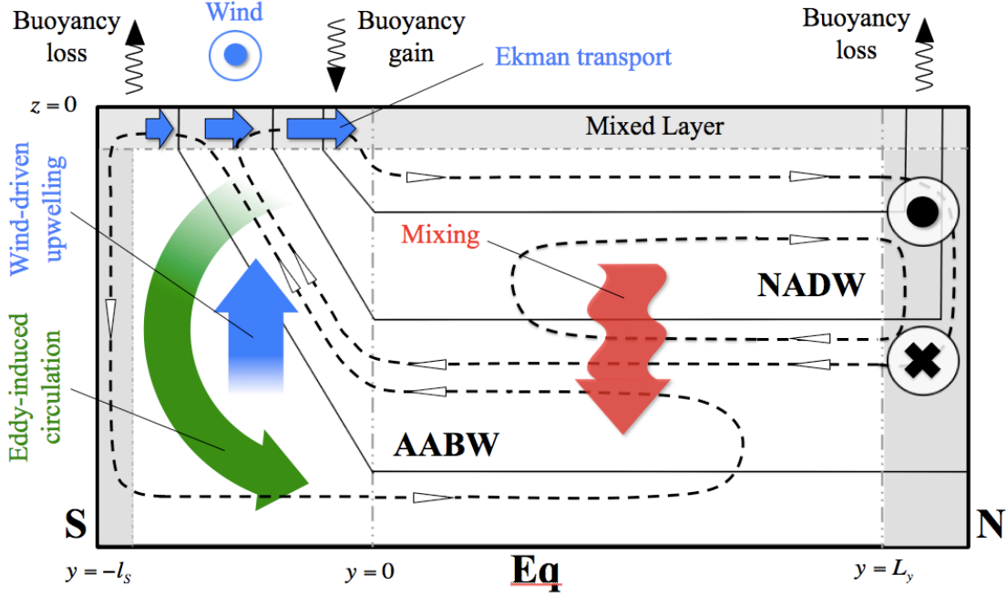
FIG. 8. Schematic of the meridional overturning circulation. Thin solid black lines are the isopycnals, thicker dashed black lines with arrows are the overturning streamlines of the residual circulation, dashed vertical lines are the boundaries between adjacent regions, shaded gray areas are the convective regions at high latitudes and the surface mixed layer.
