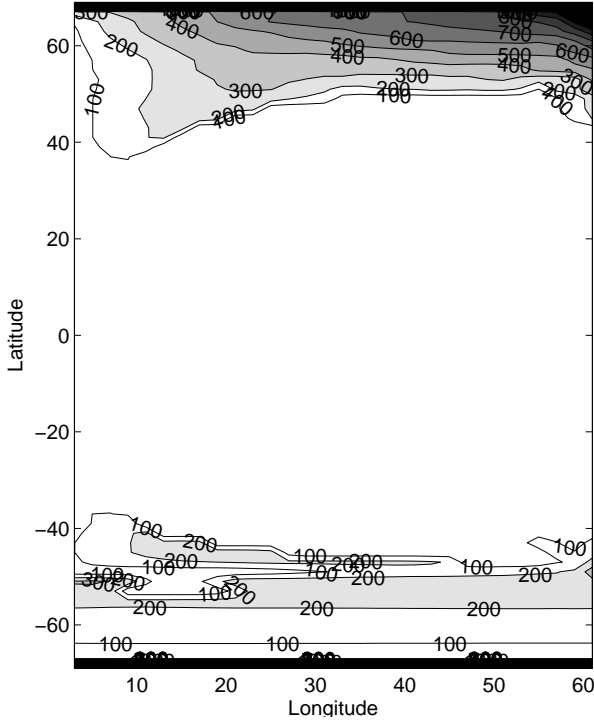
FIG. 7. Mixed layer depth (m) diagnosed from idealized GCM simulation.
