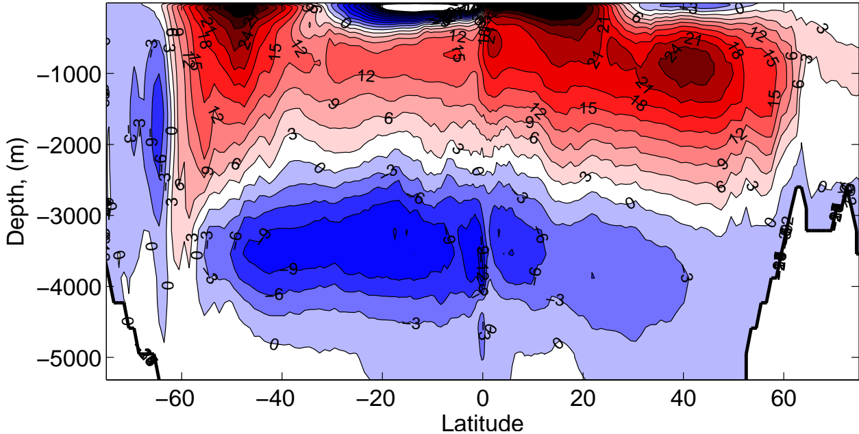
FIG. 2. Global zonally-averaged meridional overturning circulation (Sv) from the Geophysical Fluid Dynamics Laboratory Earth System Model (Dunne et al. 2012).
