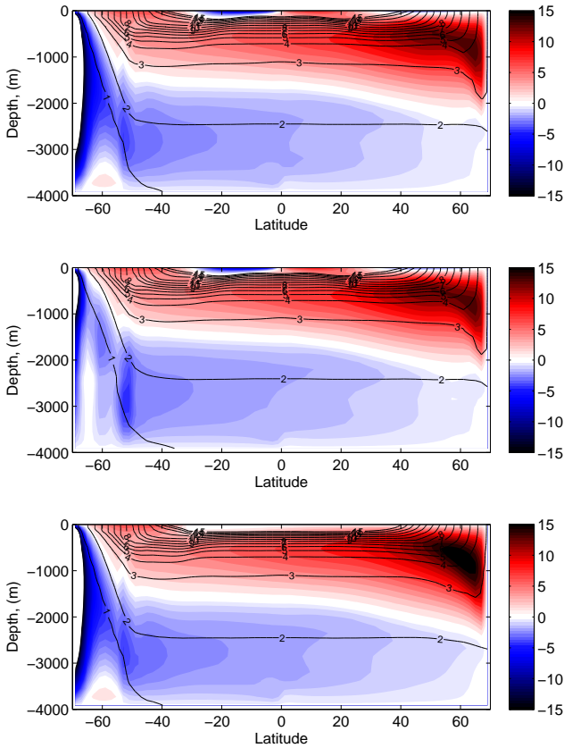
FIG. 5. Zonally-averaged temperature ( ^{\circ} C, black lines) and meridional overturning streamfunction ( S_v , blue/red) diagnosed from idealized GCM simulation from the control experiment (top panel), experiment with a 1.5 km tall ridge in the circumpolar channel (middle panel), and experiment with zero wind stress north of 30^{\circ} S (lower panel).
