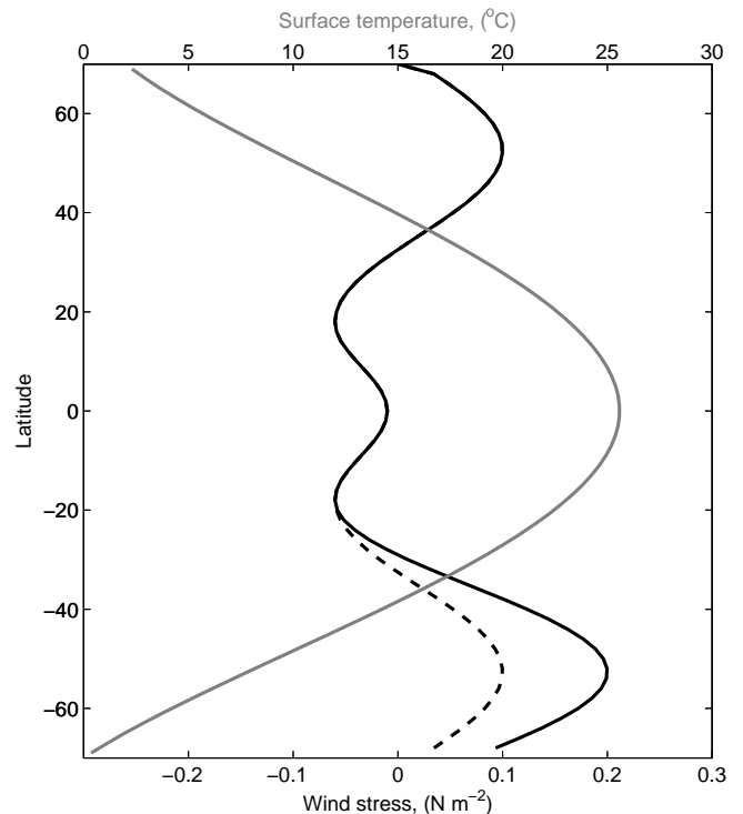
FIG. 4. The idealized mean zonally uniform wind stress (black, \text{N m}^{-2} ) and surface temperature restoring field ( ^\circ\text{C} , gray). Perturbed wind over the Southern Ocean is shown in dashed black line.
