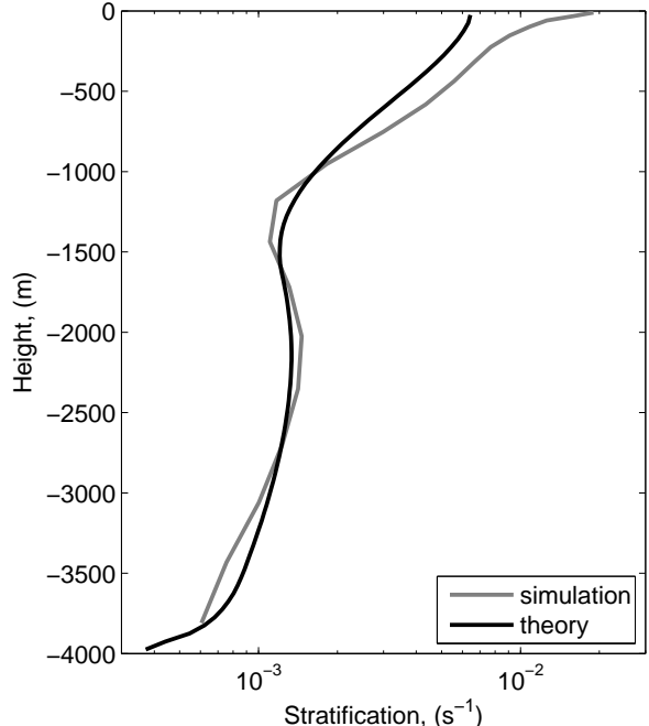
FIG. 10. Vertical profiles of stratification ( \text{s}^{-1} ) estimated from the idealized GCM simulation (gray) as an average over a low-latitude region from 30^\circ\text{S} to 30^\circ\text{N} and from theory (black).
