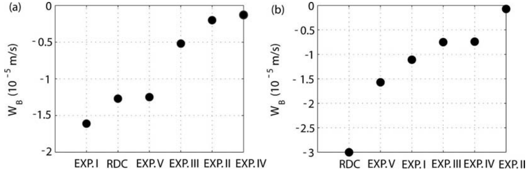
FIG. 9. Plot of averaged bottom vertical velocity W_B ( 10^{-5} m s ^{-1} ) from all experiments. (a) Around the western boundary near Grand Banks ( 44^{\circ} – 45^{\circ} N, 47^{\circ} – 46^{\circ} W). (b) Around the crossover of Gulf Stream and DWBC near Cape Hatteras ( 36^{\circ} N, 73^{\circ} – 72^{\circ} W). RDC: robust diagnostic calculation; experiments I–V same as in Fig. 8.
