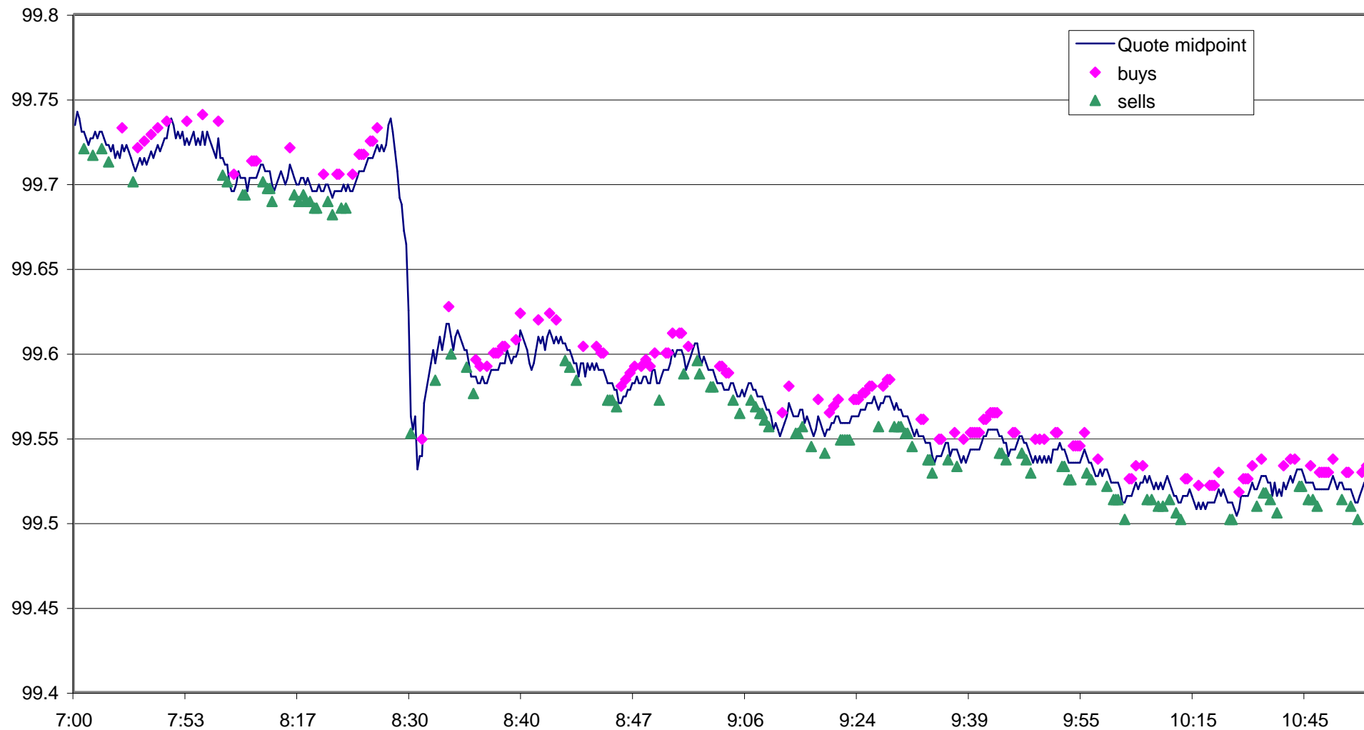
Graph 9. Quotes and transactions in the two-year note: Jan 28, 2000, 7:00-11:00 am
