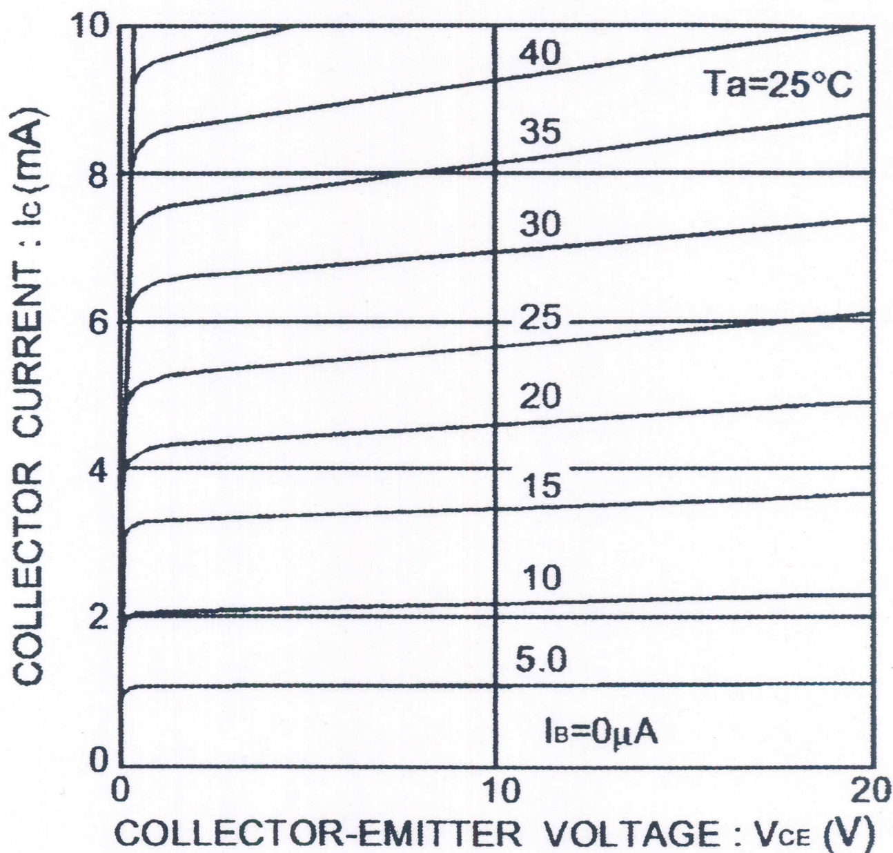
Fig.1 Grounded emitter output characteristics
