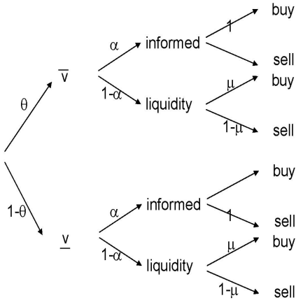
Figure: Tree.
