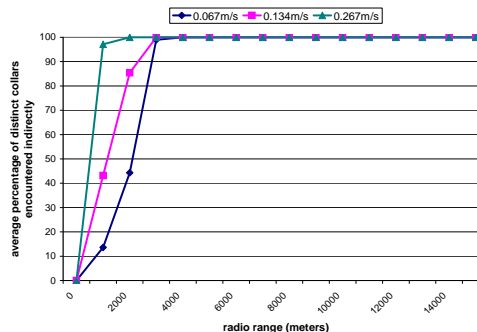
Figure 9: Average percentage of distinct nodes encountered indirectly, through peer-to-peer relaying.
