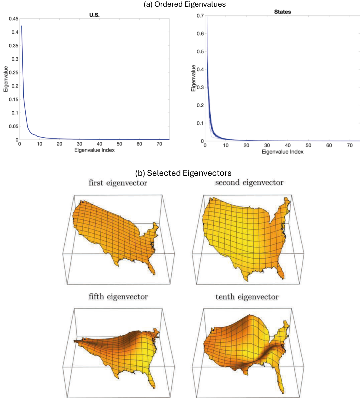
Figure 2: Eigenvalues and Eigenvectors of \bar{\Sigma}_L
