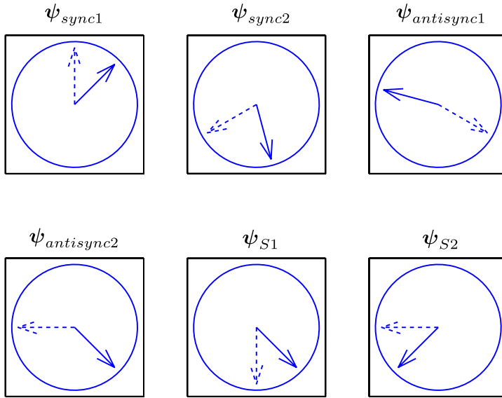
Fig. 9 These diagrams show the pictures of all the equilibria for \bar{\theta}_2 = \frac{3\pi}{4} . This is representative of the possible equilibria for the system in Region 1B without its boundary, i.e., for \bar{\theta}_2 \in (\frac{\pi}{2}, \pi) . The two saddles, \psi_{S1} and \psi_{S2} , tend to be more synchronized (than in Fig. 7) since \bar{\theta}_2 is closer to \pi . \psi_{S1} is closer to the preferred direction of the first subgroup and \psi_{S2} is closer to the preferred direction of the second subgroup. There are two stable equilibria, \psi_{sync1} and \psi_{sync2}
