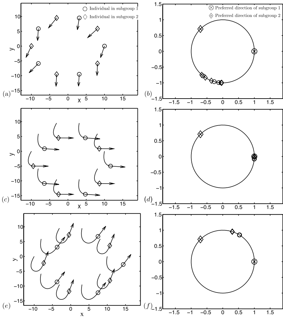
Fig. 13 Simulation for two informed subgroups each with a population of five individuals ( N_1 = N_2 = 5 ). The plots in the left column show snapshots in the physical plane of the individual positions r_j , j = 1, \dots, 10 (circles for individuals in subgroup 1 and diamonds for individuals in subgroup 2) and individual headings \theta_j , j = 1, \dots, 10 (arrows). The plots in the right column show the individual headings plotted on the unit circle together with the two preferred directions. The headings of the individuals are initially near the (unstable) equilibrium \psi_{\text{sync}2} with K = 70 , \bar{\theta}_2 = \frac{3\pi}{4} . (a) and (b) correspond to initial time t = 0 . (c) and (d) correspond to time t = 11.73 . (e) and (f) correspond to time t = 19.16
