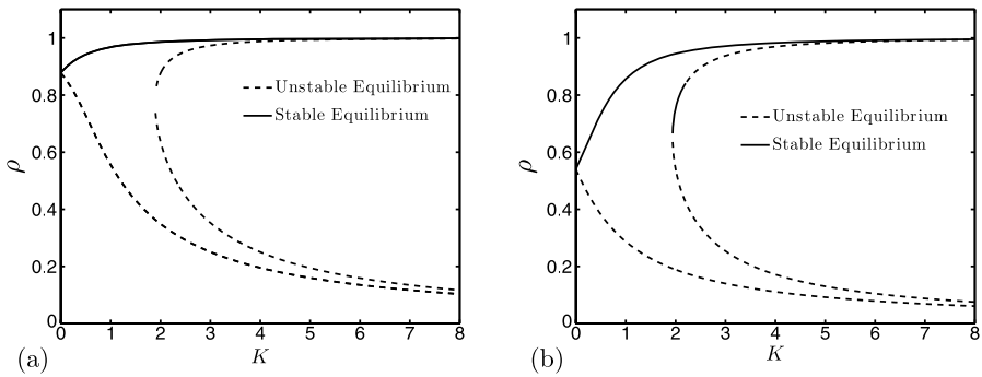
Fig. 3 Bifurcation diagrams in cases (a) \bar{\theta}_2 = 1 rad and (b) \bar{\theta}_2 = 2 rad. The bifurcation parameter is K and \rho is plotted as a function of K for all equilibria in the second set of solutions. We note that two equilibria do not exist for low values of K . Stability of these same two equilibria changes type between (a) and (b), indicating the presence of bifurcations
