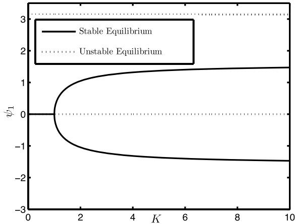
Fig. 11 Bifurcation diagram in the (K, \Psi_1) plane, i.e., \Psi_1 as a function of bifurcation parameter K fixing \theta_2 = \pi . At K = 1 , we have a supercritical pitchfork bifurcation. We have one stable equilibrium for K < 1 and two stable equilibria for K > 1
