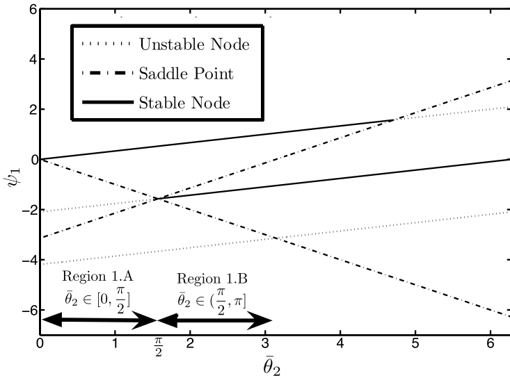
Fig. 6 Bifurcation diagram in the (\bar{\theta}_2, \Psi_1) plane, i.e., \Psi_1 as a function of bifurcation parameter \bar{\theta}_2 fixing K = 2 . Since the equilibria \psi_{\text{antisync2}} and \psi_{S1} have the same value for \Psi_1 (but a different value for \Psi_2 ), we see on this diagram only 5 equilibria even though there are six. At \bar{\theta}_2 = \frac{\pi}{2} , there are only three distinct equilibria; this is the degenerate point of the system. The multiplicity of the equilibrium (\frac{3\pi}{2}, \pi) is four
