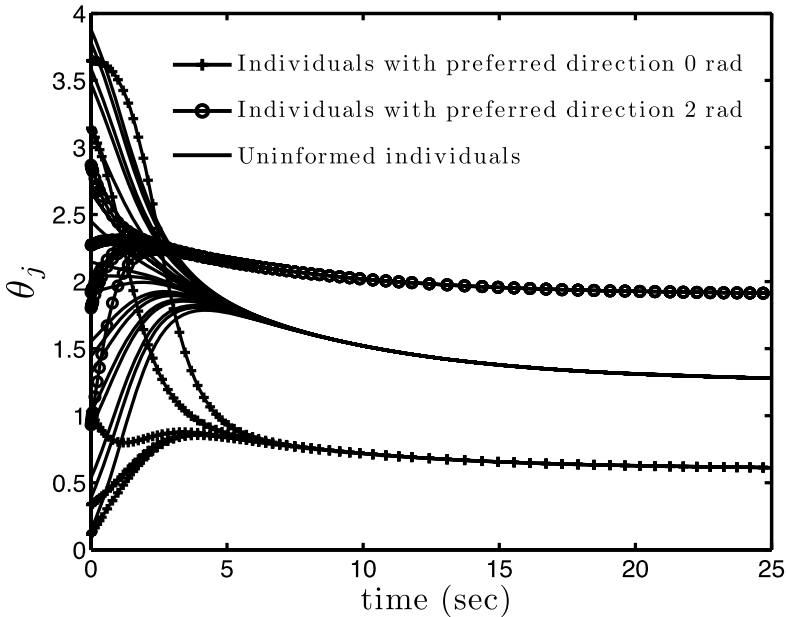
Fig. 1 Phase angle of each individual in the group versus time for K = 1 . For this simulation, there are 5 individuals with preferred direction 0 rad, 5 individuals with preferred direction 2 rad, and 20 individuals with no preferred direction. Two time scales in the dynamics can be observed. During a short initial transient time, the heading angles of the individuals in each subgroup synchronize. Then the three average subgroup directions change slowly to their steady state values
