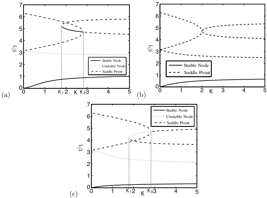
Fig. 4 Bifurcation diagrams in cases (a) \bar{\theta}_2 = \frac{3\pi}{4} , (b) \bar{\theta}_2 = \frac{\pi}{2} , and (c) \bar{\theta}_2 = \frac{\pi}{4} . The bifurcation parameter is K and \psi_1 is plotted as a function of K for all equilibria of the system. We observe the hypercritical pitchfork bifurcation for \bar{\theta}_2 = \frac{3\pi}{4} at K = K_0 . For the case \bar{\theta}_2 = \frac{\pi}{4} , the bifurcation at K = K_0 only consists of a change in the number of equilibria, but does not affect the stability of the system. In the case that \bar{\theta}_2 = \frac{\pi}{2} , the bifurcation only consists in the disappearance of two saddle points simultaneously with the appearance of two new ones
