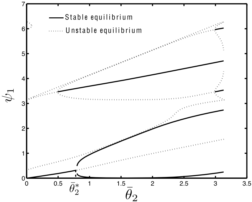
Fig. 2 Bifurcation diagrams for the system (13) with K = 2.5, \alpha = 0.2 . The bifurcation parameter is \bar{\theta}_2 and \psi_1 is plotted as a function of \bar{\theta}_2 for all equilibria of the system. We observe the supercritical pitchfork bifurcation at \bar{\theta}_2 = \bar{\theta}_2^*
