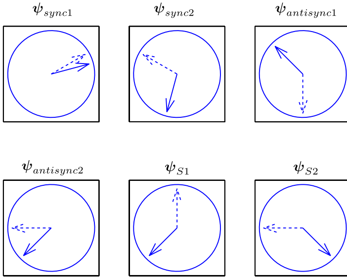
Fig. 7 These diagrams show pictures of all the equilibria for \bar{\theta}_2 = \frac{\pi}{4} . This is representative of the possible equilibria for the system in Region 1A without its boundary, i.e., for \bar{\theta}_2 \in [0, \frac{\pi}{2}) . The only stable equilibrium is \psi_{sync1} , which for this example corresponds to motion in the \Psi = \frac{\pi}{8} direction
