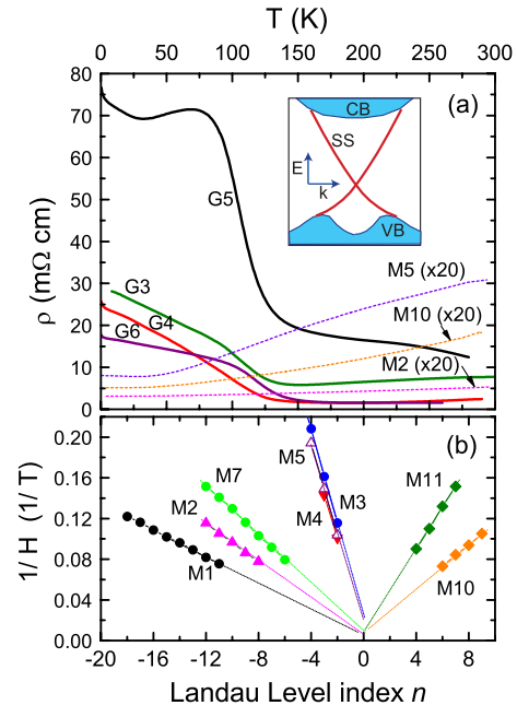
FIG. 1 (color online). (a) Resistivity \rho vs T in 4 samples (G3–G6) of \text{Ca}_x\text{Bi}_{2-x}\text{Se}_3 lightly doped with Ca to bring \mu_b into the gap. Samples with \mu_b not inside the gap (M2, M5, and M10) display a metallic T dependence (shown \times 20 ). The inset is a sketch of the surface states [8] crossing the gap from the VB to the CB. (b) The LL index plot vs field minima in the SdH oscillations observed in 8 metallic samples (M1 \cdots M11). Negative (positive) index n represents the electron (hole) FS pocket. As \mu_b is lowered from the CB to VB, the FS area S_F \sim 1/\text{slope} decreases before rising again.
