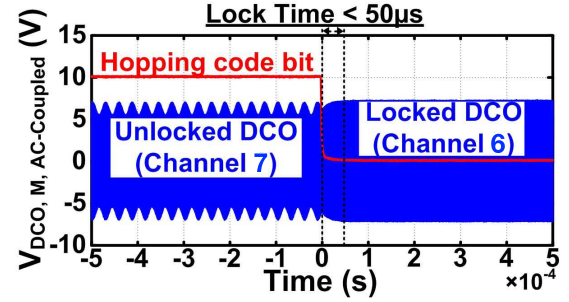
Fig. 25. Time required for DCO to lock is <50 \mu s.
