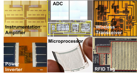
Figure 3. Recent demonstrations of TFT circuits [28,37,38,42-44].
