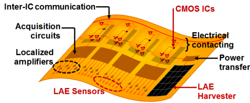
Figure 6. Illustration of hybrid-system interfacing challenges.
