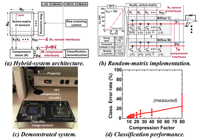
Figure 10. LAE-based feature-extraction system [61].
