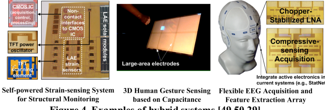
Figure 4. Examples of hybrid systems [49,50,29].
