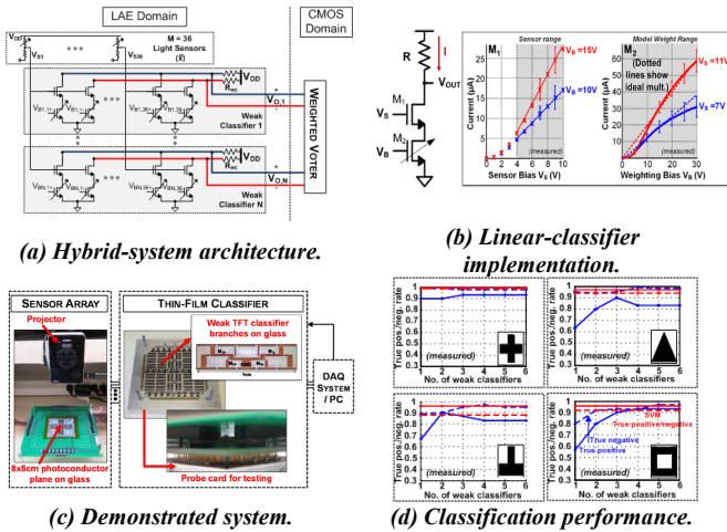
Figure 11. LAE-based classification system [35].
