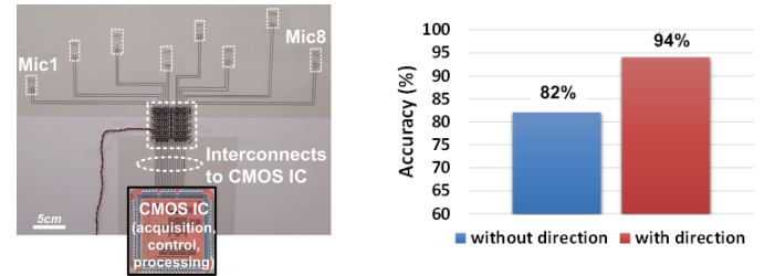
(a) Hybrid system hardware [52]. (b) Audio detection performance. Figure 5. Demonstration of large-area microphone phased array.
