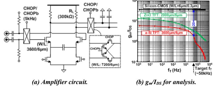
Figure 7. Low-noise TFT amplifier [29].
