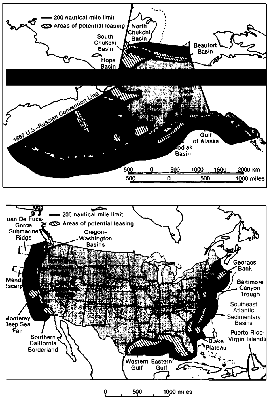
Figure 2-2.—Sedimentary Basins in the EEZ
