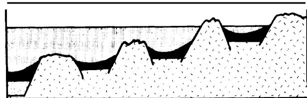
Southern California Borderland: (extensional)
