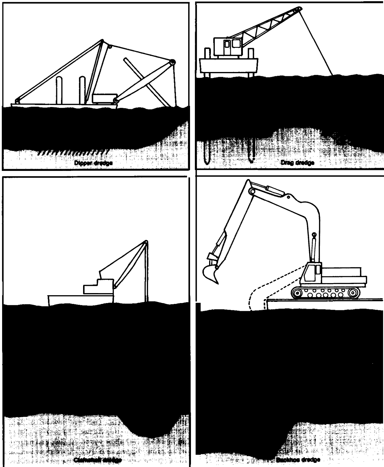
Figure 5-9.—Grab Dredges
