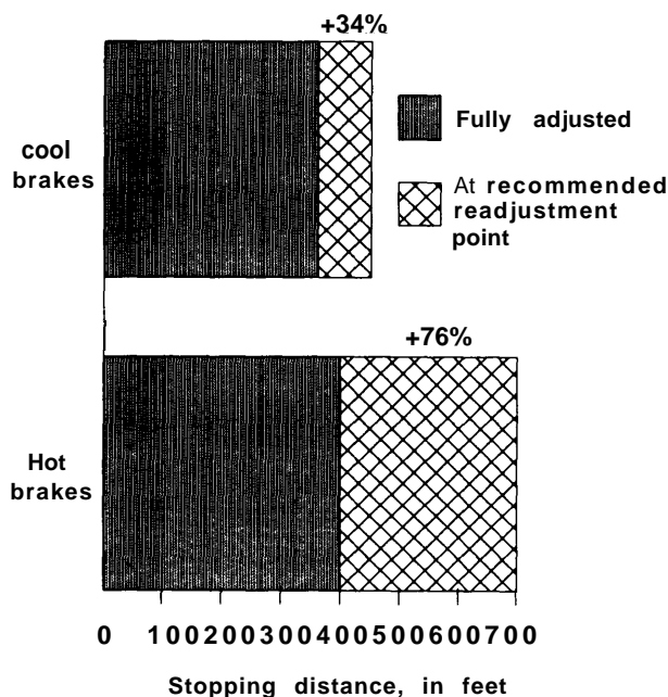
Figure 5-8.—Stopping Distance of Fully Loaded Truck at Two Brake Adjustment Levels
