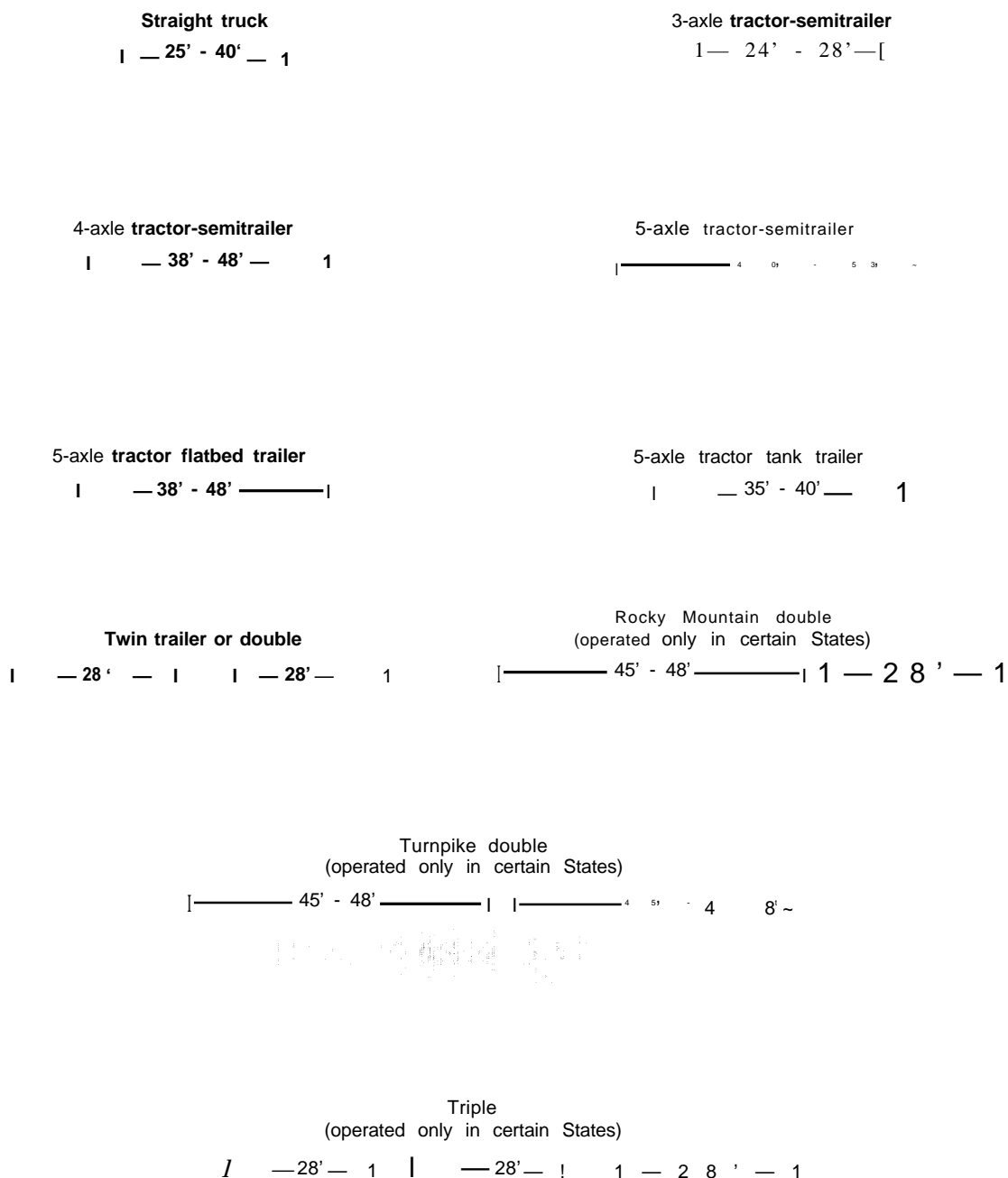
Figure 2-1.—Truck Types
