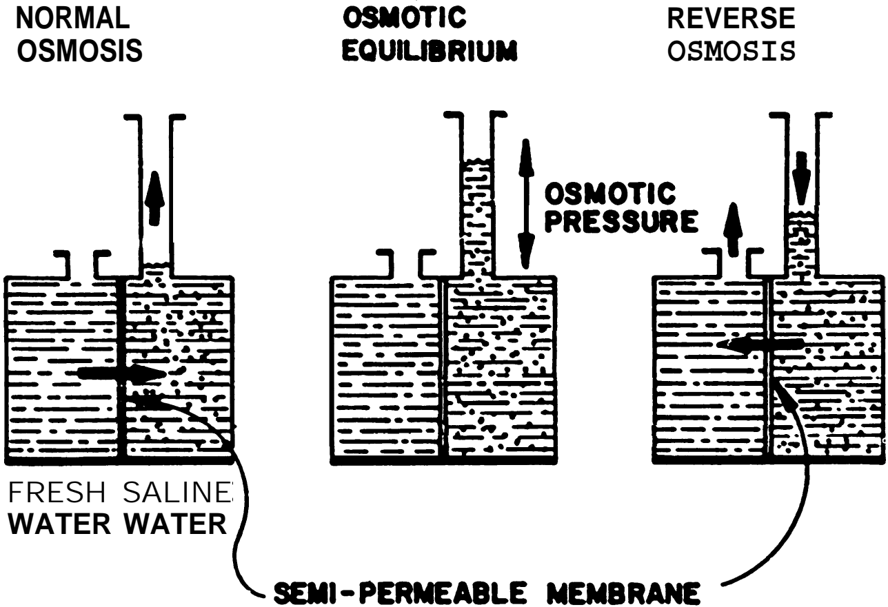
Figure 5A.—Principles of Reverse Osmosis
