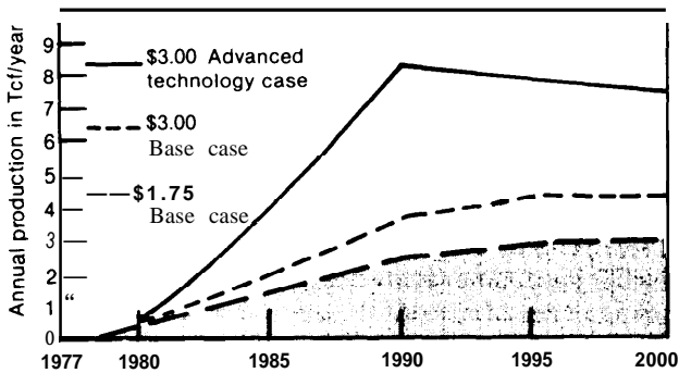
Figure 5.—Annual Production From Unconventional Sources to the Year 2000 at $1.75 and $3.00/Mcf (except geopressedured aquifers)
