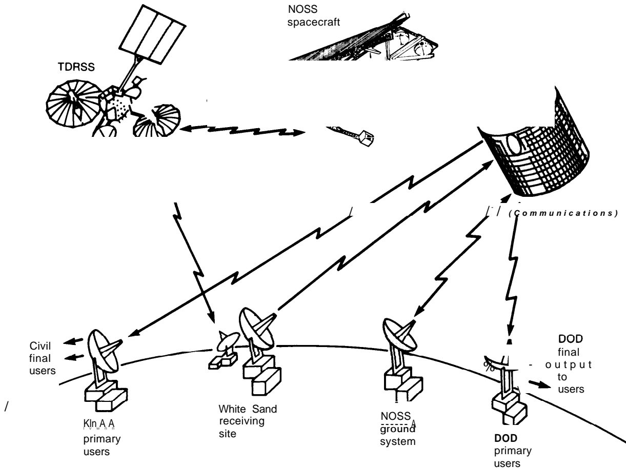
Figure 19.—NOSS End-to-End System
