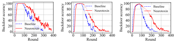
Figure 4. Attack accuracy of baseline and Neurotoxin on Reddit dataset with LSTM with different length trigger sentence. (Left) Trigger len = 3, means the trigger sentence is “{race} people are*”, (Middle) trigger len = 2, means the trigger sentence is “{race} people*”, and (Right) trigger len = 1, means the trigger sentence is “{race}***”, where “race” is a random word selected from {black yellow white brown} and “*” is the target word. Start round and AttackNum of all experiments are 1800 and 80, respectively. The Lifespan of the baseline and neurotoxin are (Left) 78 and 123, (Middle) 54 and 93, (Right) 32 and 122.
